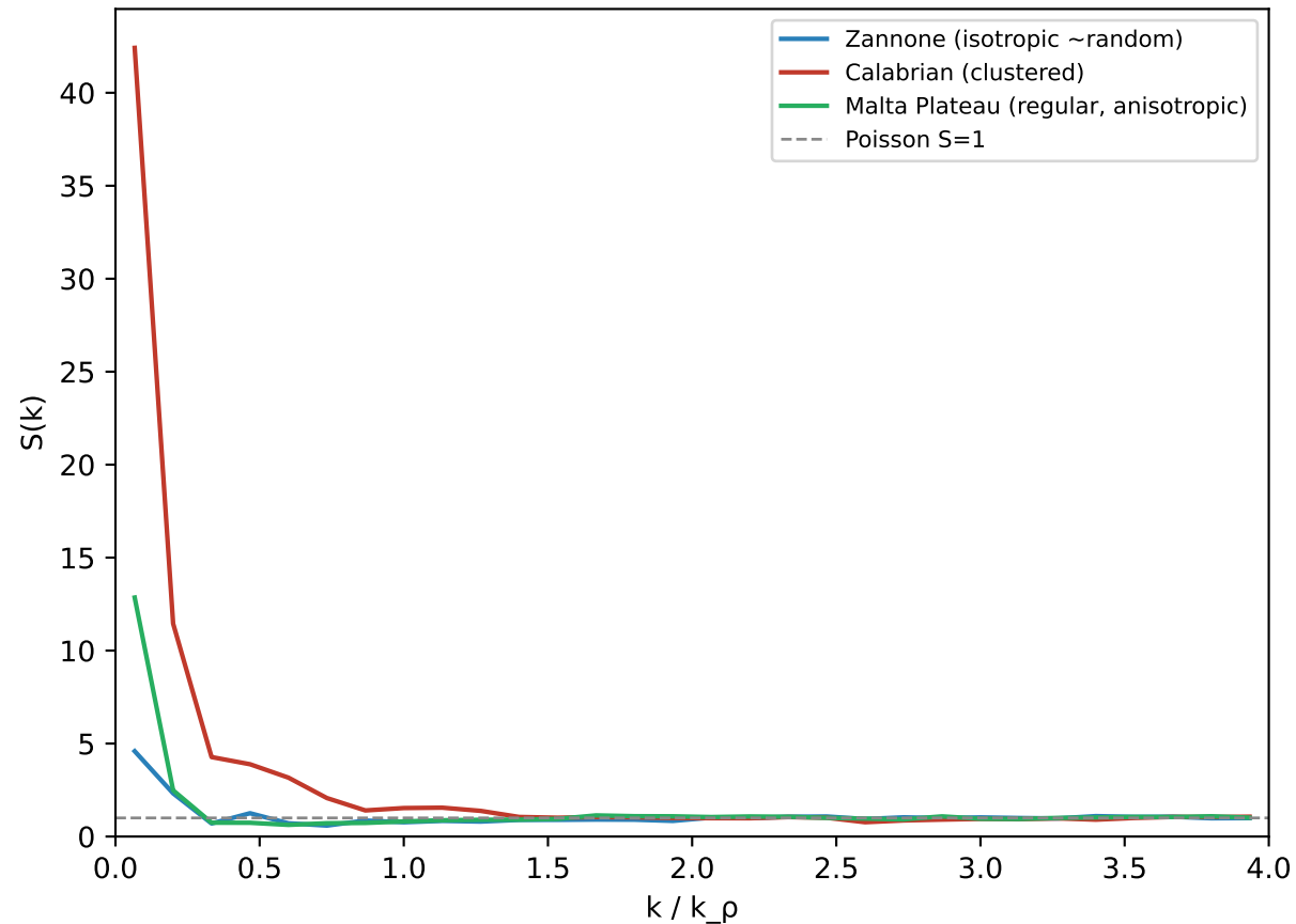
(b) radial structure factor: low-k rises above 1 (heterogeneity); no S(k \rightarrow 0) \rightarrow 0 hyperuniform dip
