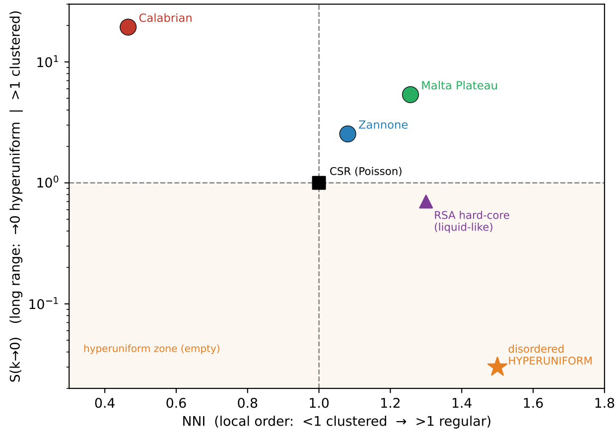
(a) order plane: local order varies, but every field is long-range super-Poissonian — none hyperuniform
