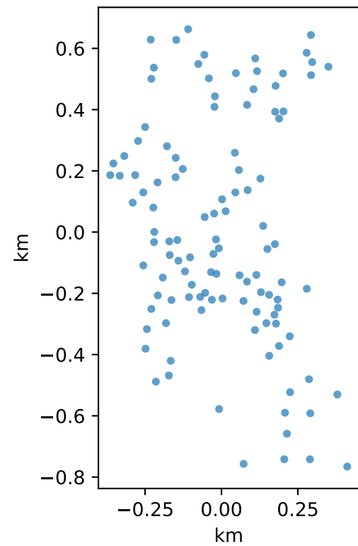
Zannone (isotropic \sim random) N=112, NNI=1.08
