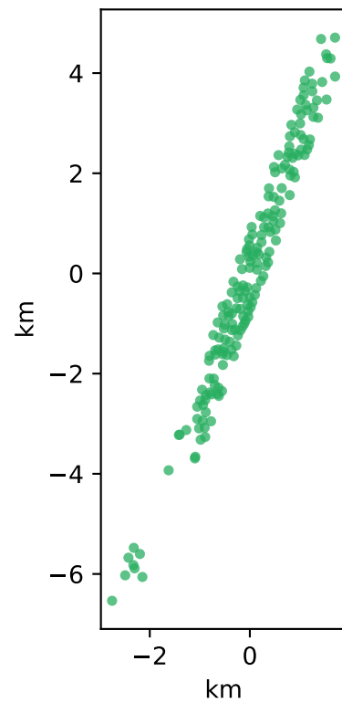
Malta Plateau (regular, anisotropic) N=184, NNI=1.26
