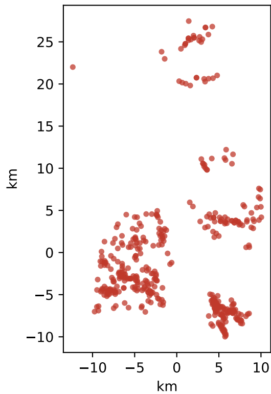
Calabrian (clustered) N=418, NNI=0.47
