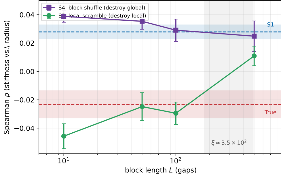
Figure 5: The S4/S5 scissors at N = 10^4 , n = 40 per arm. Spearman \rho (stiffness vs. radius) against block length L , with the true-prime and shuffle (S1) reference bands (mean \pm s.e.m.). S4 (block shuffle; destroy global order, keep local) remains statistically pinned to the shuffle band at every L (vs. S1: p \geq 0.10 ). S5 (local scramble; destroy local order, keep global) remains pinned to the true-prime band up to L \approx 10^2 (vs. true at L = 50, 100 : p = 0.91, 0.62 ) and departs toward the shuffle only for L \gtrsim \xi . The two blades cross near the half-retention scale \xi \approx 3.5 \times 10^2 gaps (shaded, 68% CI [1.8, 4.9] \times 10^2 ), the correlation length over which the core-shell ordering collapses.
