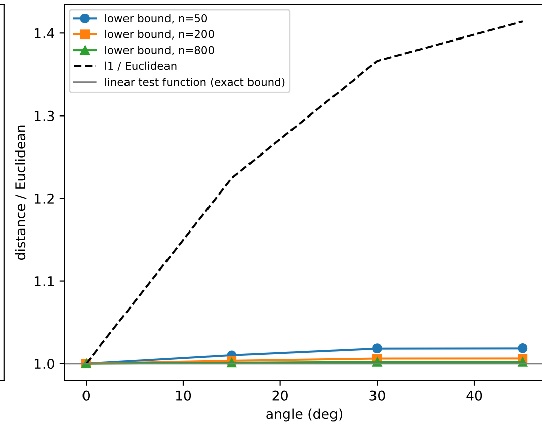
Connes distance on the square lattice
