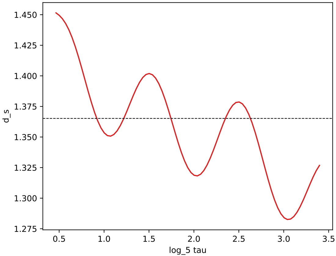
Sierpinski gasket: log-periodic d_s (period \ln 5 )
