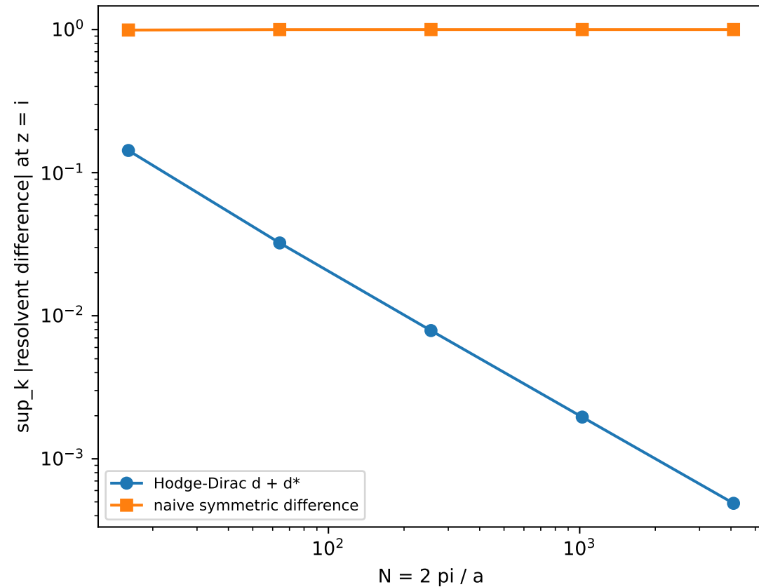
Norm-resolvent convergence vs fermion doubling
