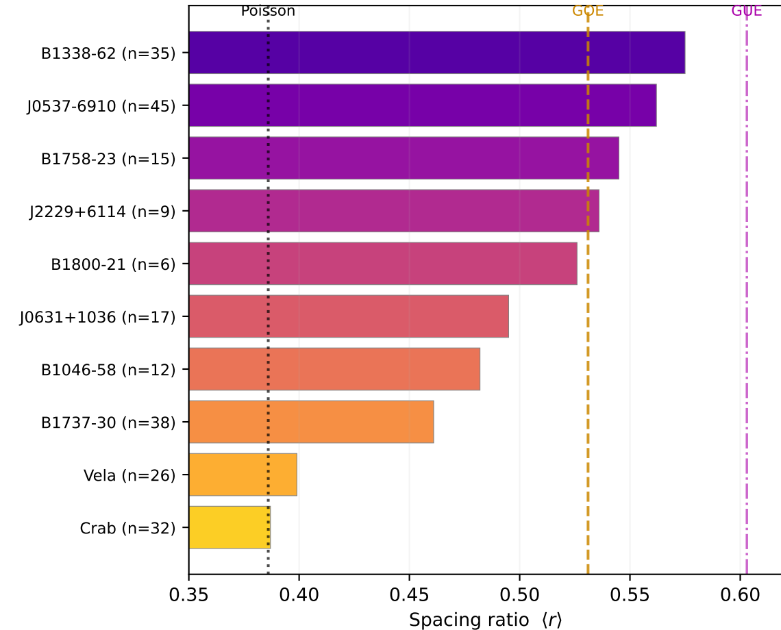
(a) The glitch memory spectrum
