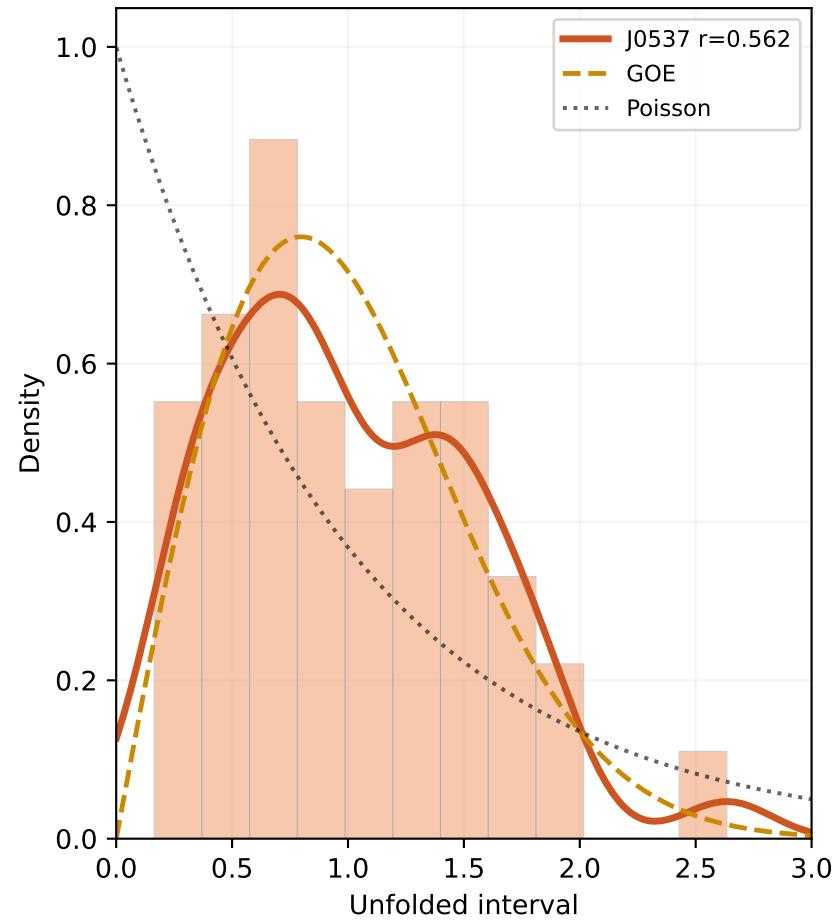
(b) J0537-6910: clean GOE (+3.6 sigma)
