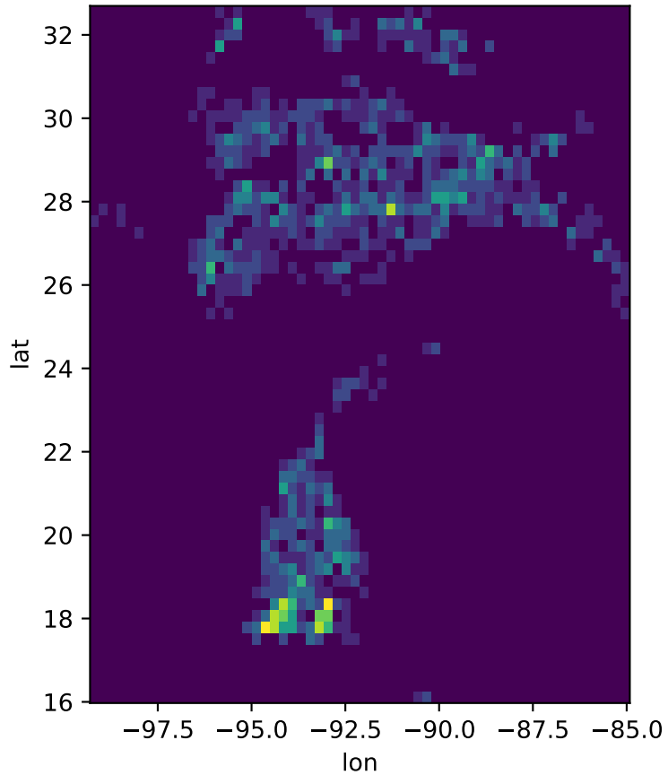
binned counts (sub-basins / gradient)
