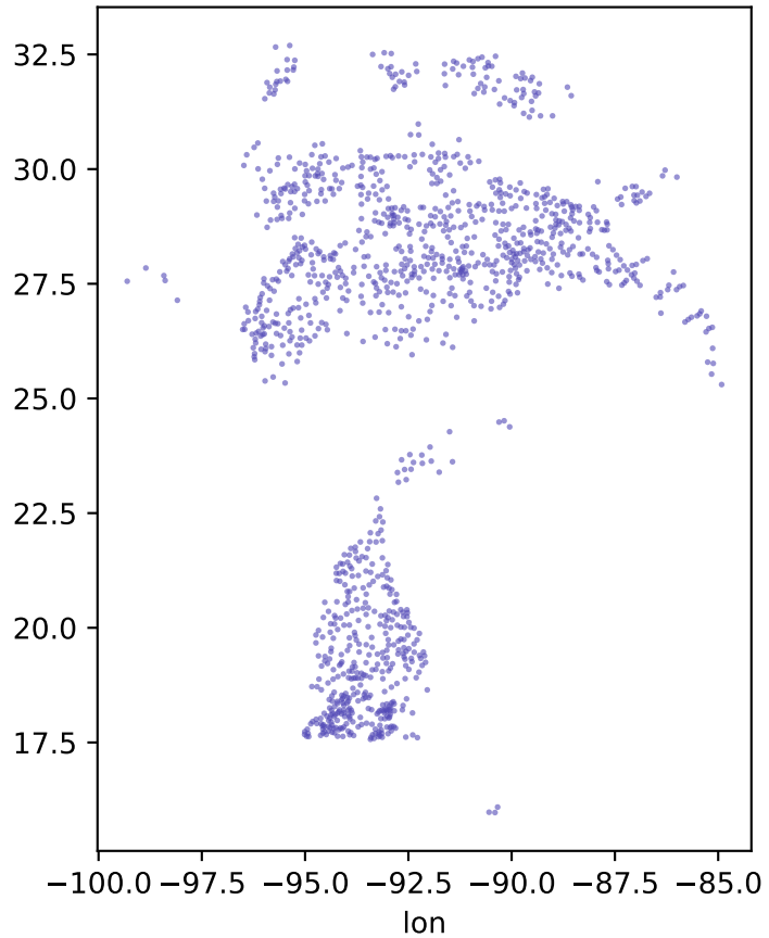
Gulf Coast salt diapirs (N=1253)
