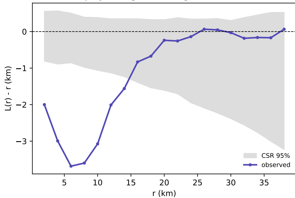
Ripley L: negative = regular ( R=1.41 )
