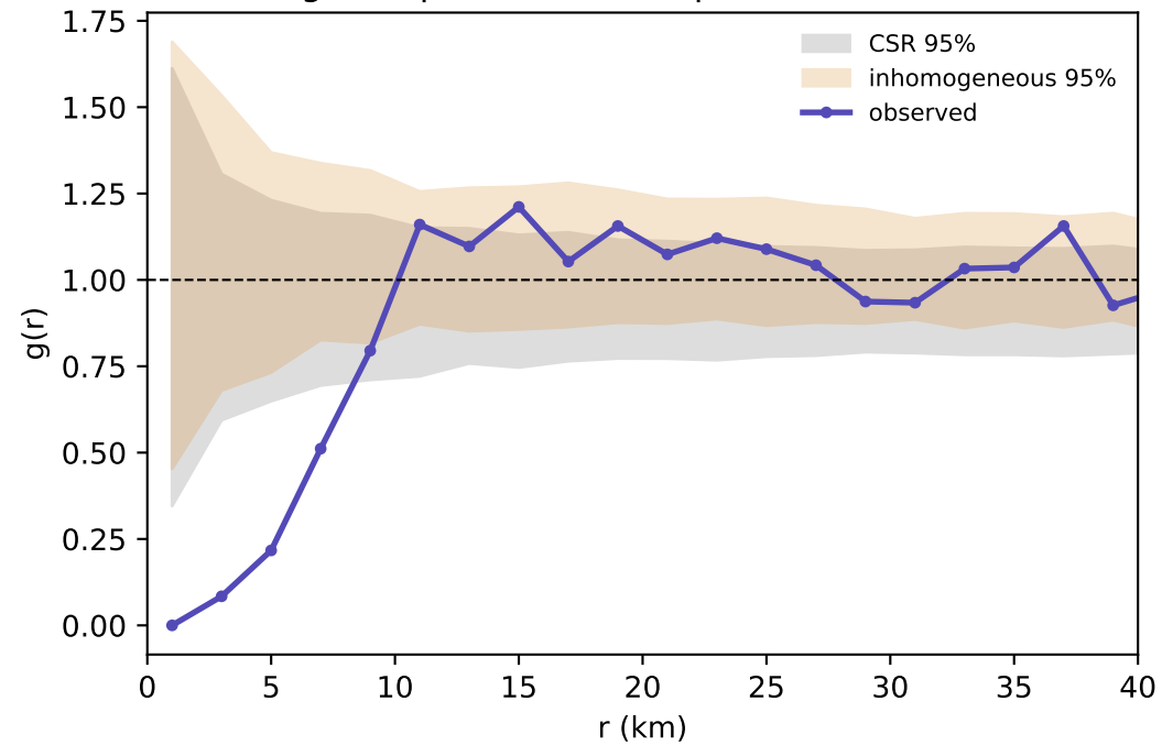
g(r) : hard-core + characteristic spacing global p(\text{CSR})=0.001 , p(\text{inhom})=0.003
