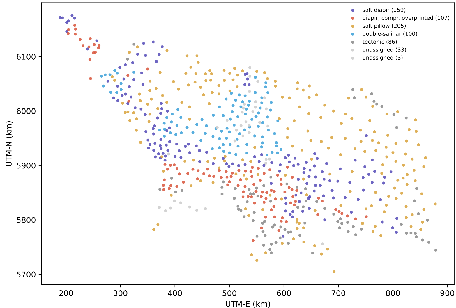
North German salt structures by internal type
