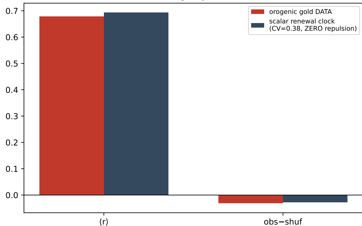
(b) A zero-repulsion scalar clock reproduces BOTH the \langle r \rangle=0.68 and the -0.03 'rigidity' (a normalization artifact)
