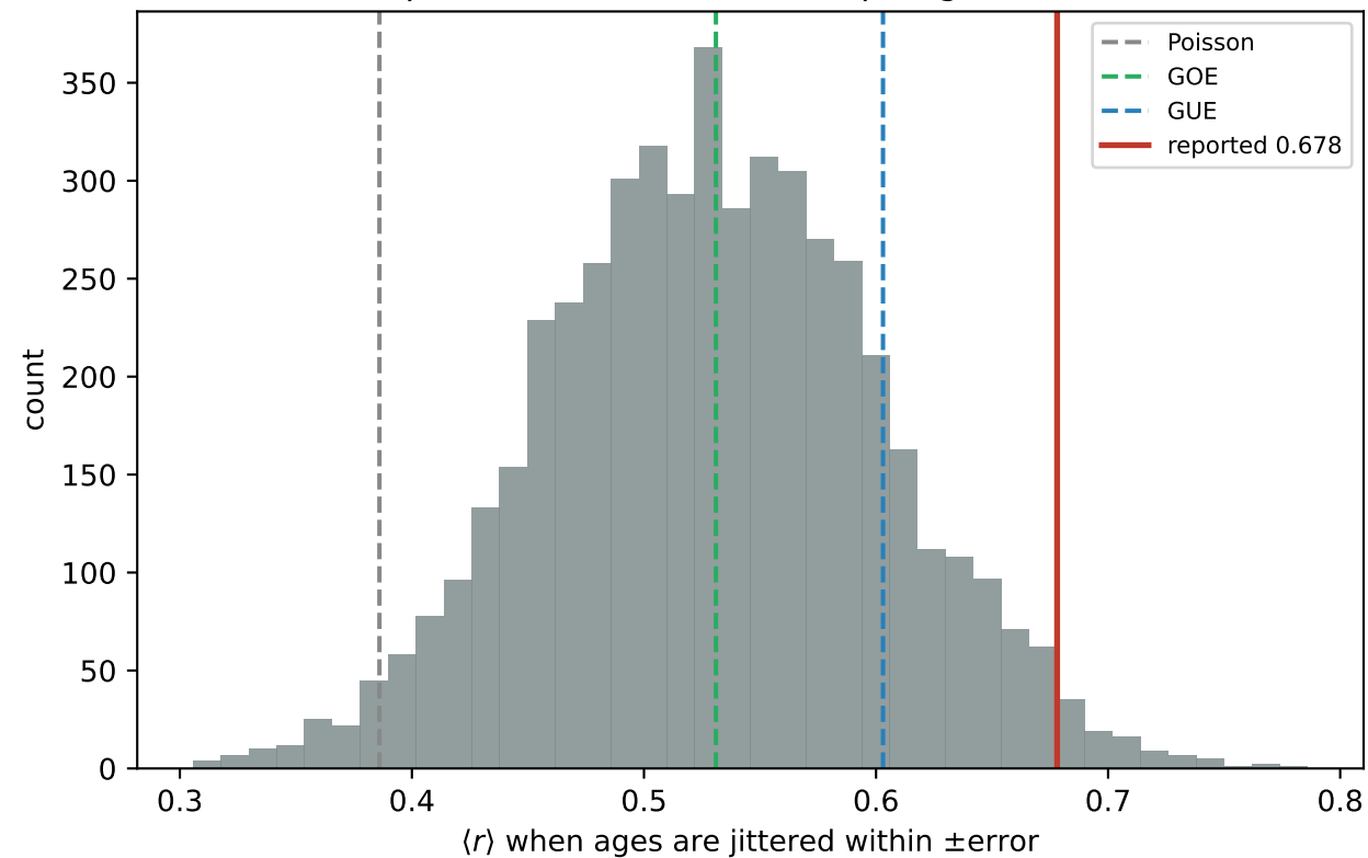
(a) Age errors alone move \langle r \rangle across Poisson→GUE; the reported value sits at the top edge of the noise
