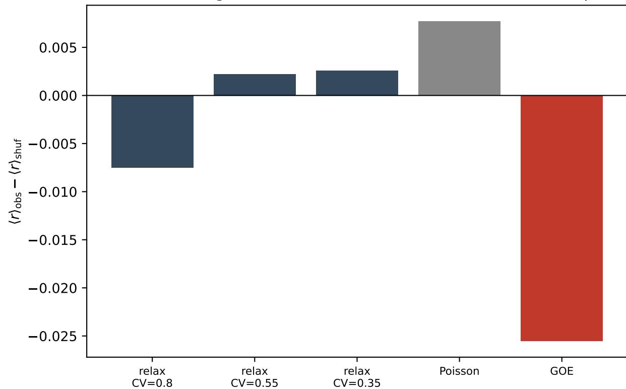
(b) Only genuine GOE has the negative rigidity signature; renewal clocks give \text{obs} - \text{shuf} \approx 0 (and need N \gg 300 to tell apart)
