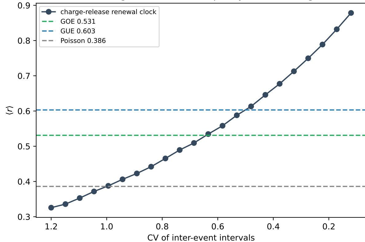
(a) A relaxation-oscillator (renewal) clock reproduces ANY \langle r \rangle — including GOE and GUE — purely from its marginal CV
