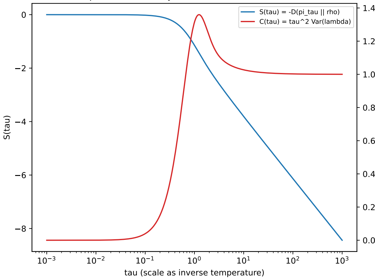
Spectral thermodynamics of scale (2D lattice)
