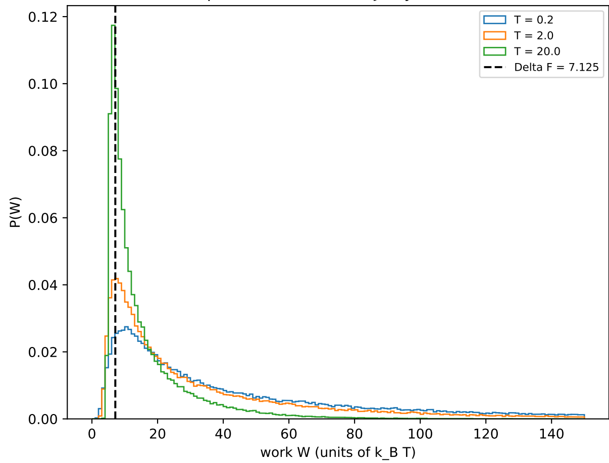
Scale protocol \xi: 10 \rightarrow 1 (Jarzynski, Crooks)
