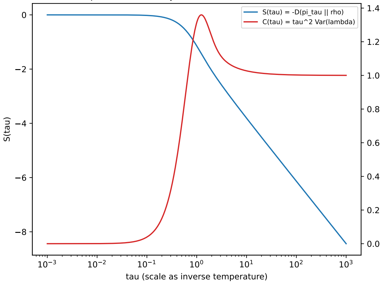
Spectral thermodynamics of scale (2D lattice)
