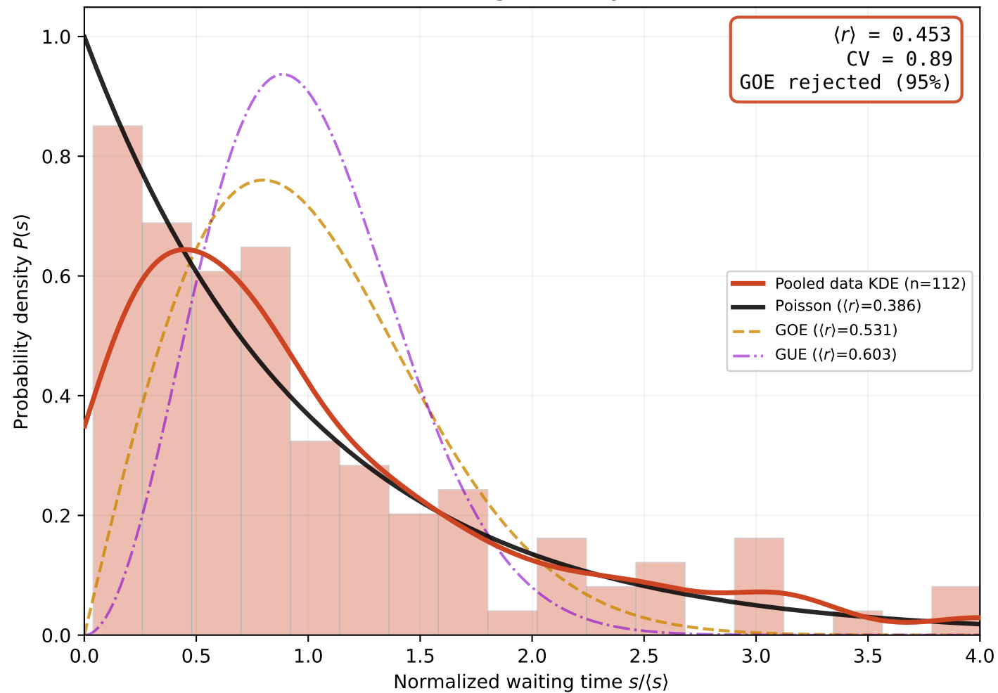
(a) Pooled 5 Active Regions — Real GOES M/X (112 waiting times, Cycle 24)
