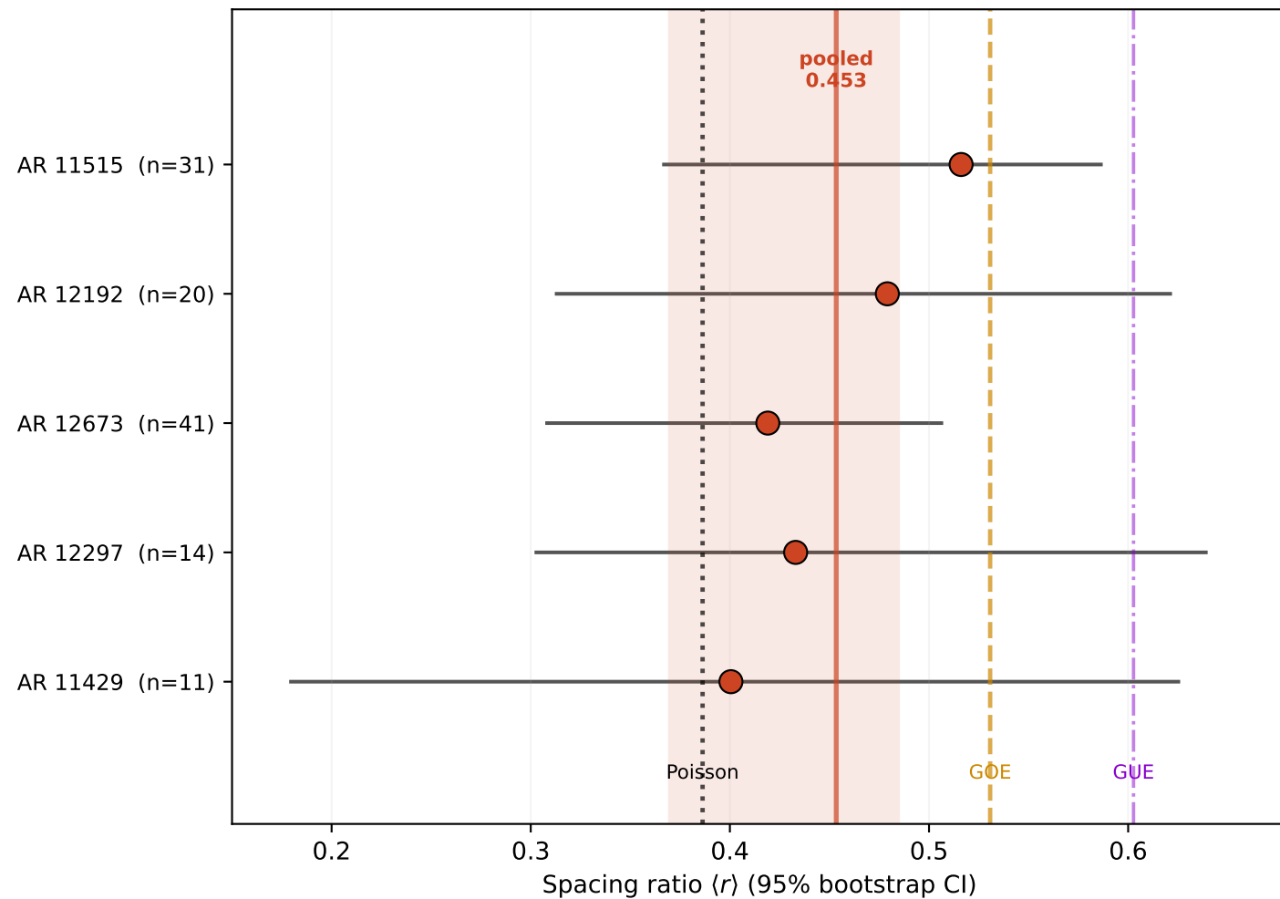
(b) Per-Region \langle r \rangle : Scatter, but Pooled Excludes GOE
