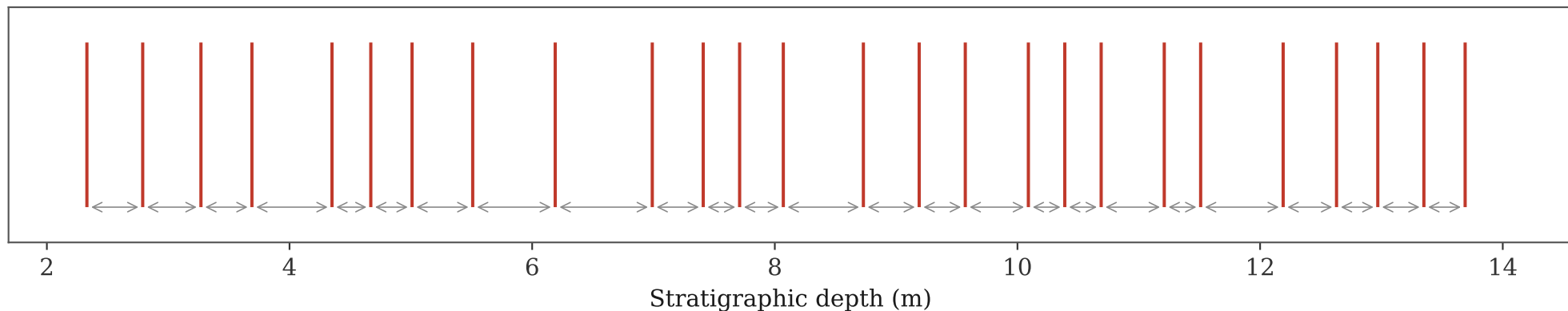
Spatial spacings \Delta Z between consecutive cycles \rightarrow RMT analysis
