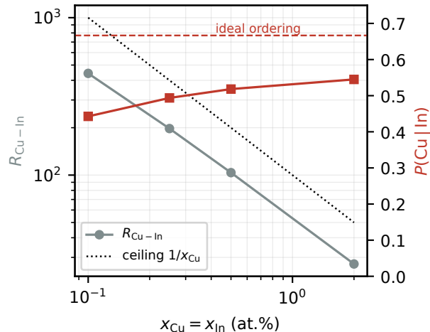
(a) enrichment factor vs shell composition
