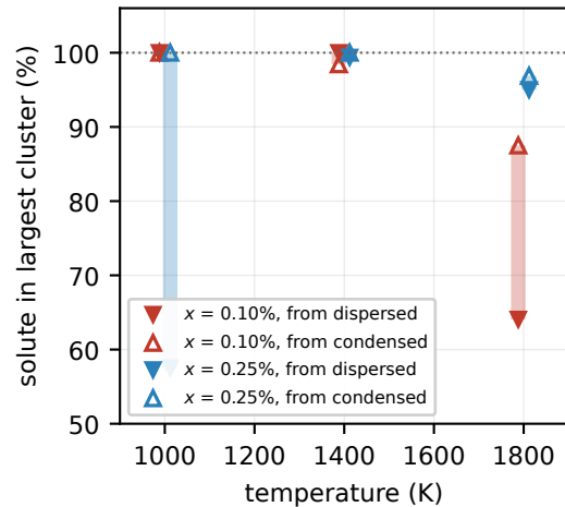
(c) equilibrium bracketed from both sides
