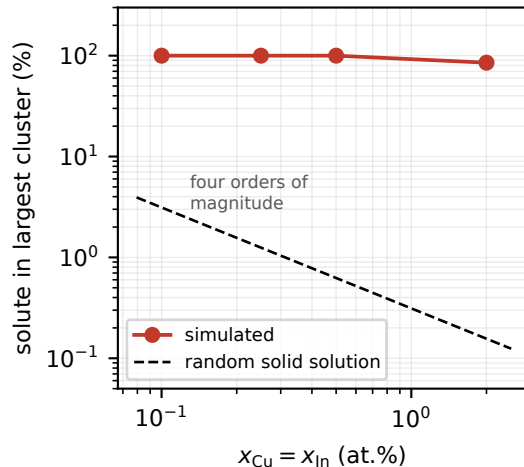
(b) condensation across the scan
