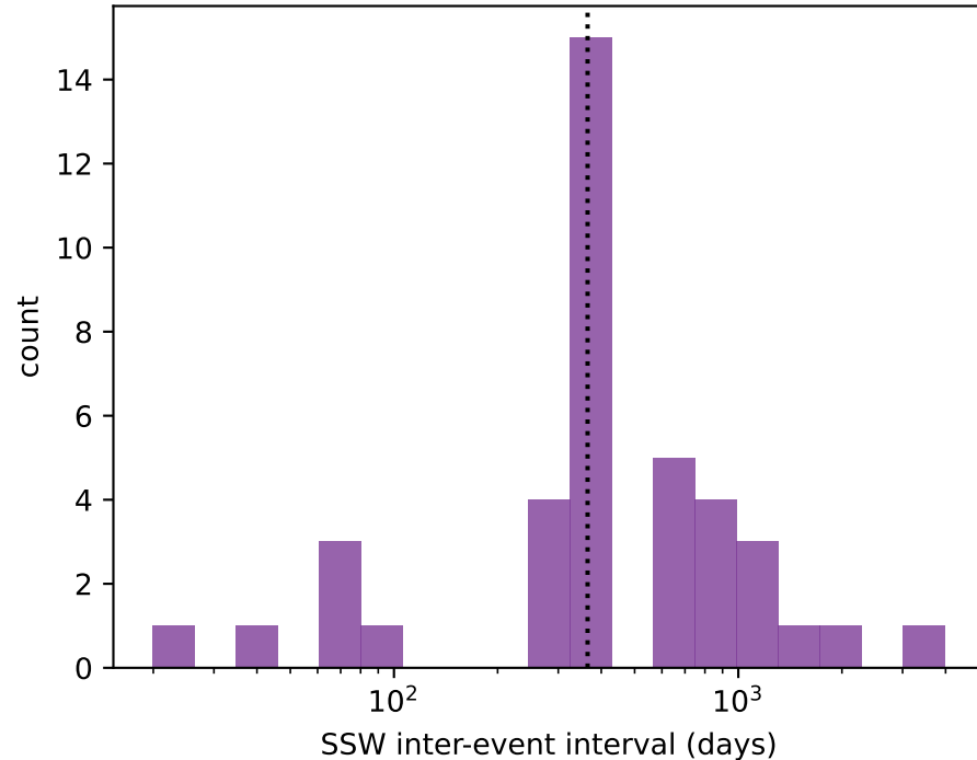
(b) Hazard 2: seasonal gating bimodal intervals; naive \langle r \rangle = 0.48 (=shuf, artifact)
