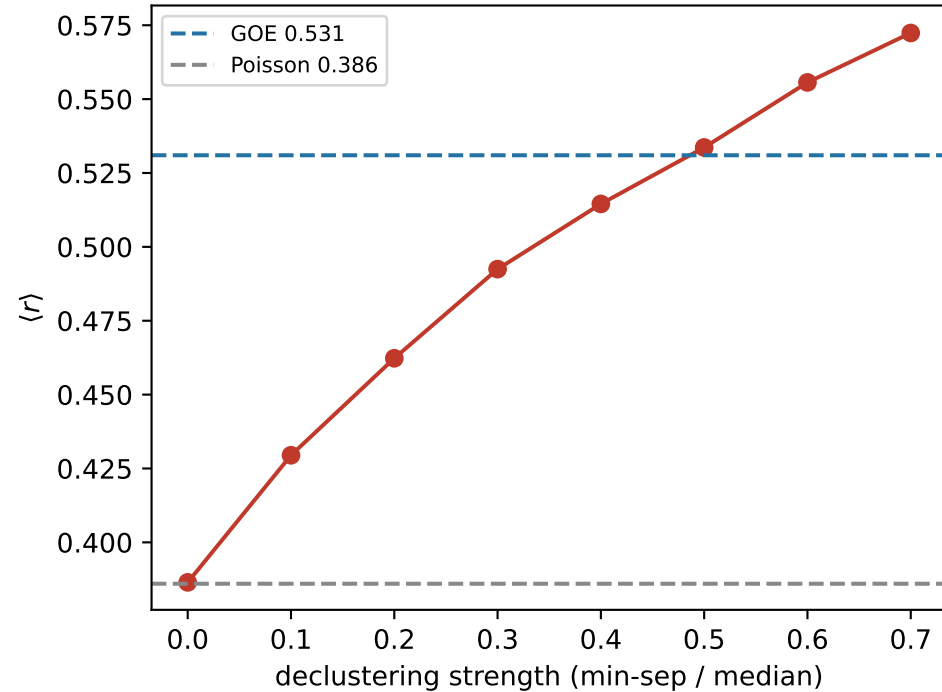
(a) Hazard 1: declustering fabricates GOE (input = pure random points)
