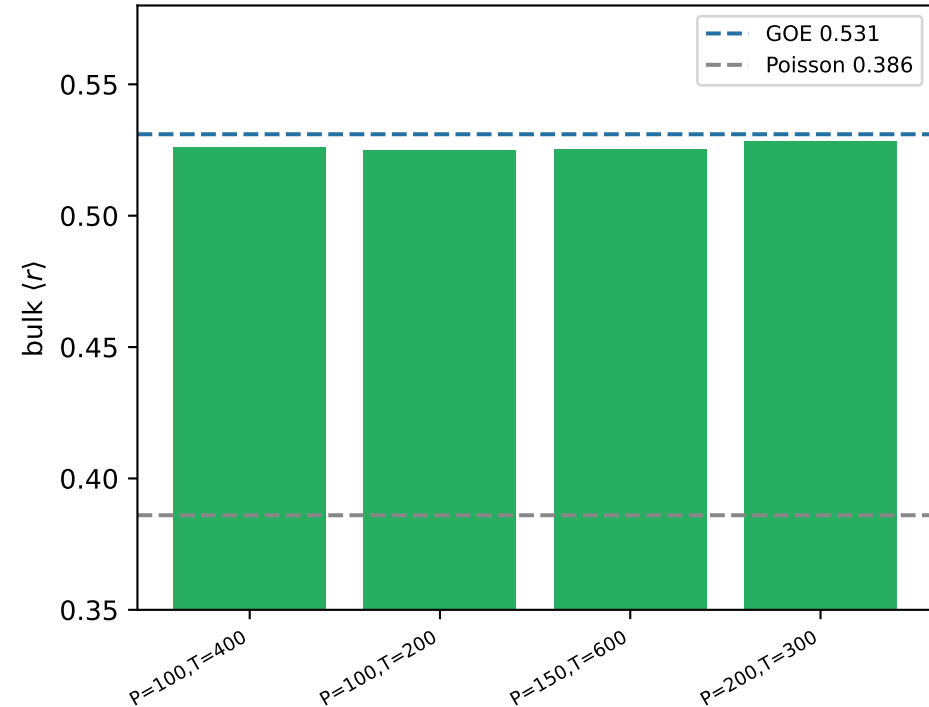
(c) Hazard 3: Wishart null (iid data \rightarrow sample corr. matrix \rightarrow GOE)
