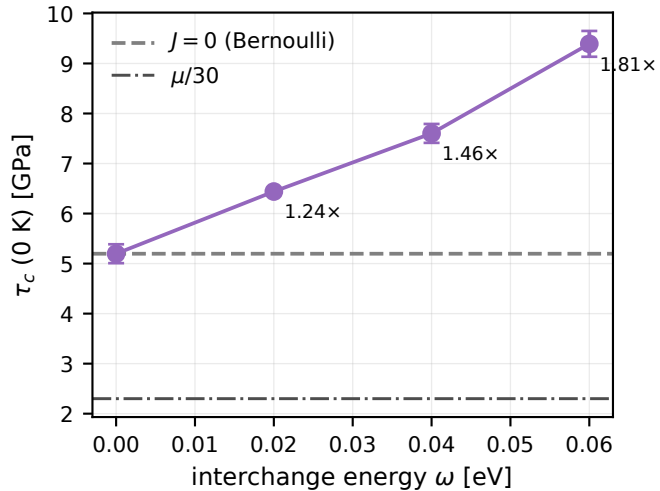
(b) solute-solute interaction, \theta = 1
