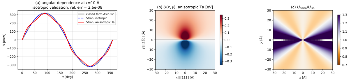
Figure 1: Solute-dislocation interaction from the elastic dipole tensor. (a) angular dependence at r = 10 Å; the isotropic Stroh solution reproduces the closed form A \sin \theta / r to 2.6 \times 10^{-8} . (b) anisotropic field of the edge dislocation. (c) ratio of anisotropic to isotropic: the amplitude changes by only -1.8\% but the angular shape deviates by up to \pm 30\% near the glide plane, which is where dU/dx controls pinning.
