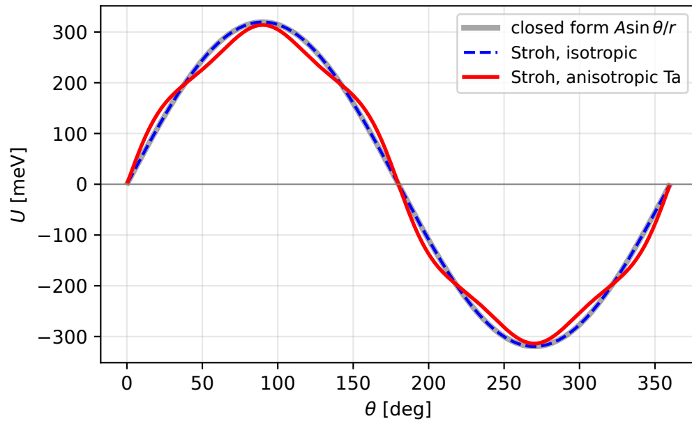
(a) angular dependence at r=10 \text{ \AA} isotropic validation: rel. err = 2.6\text{e-}08
