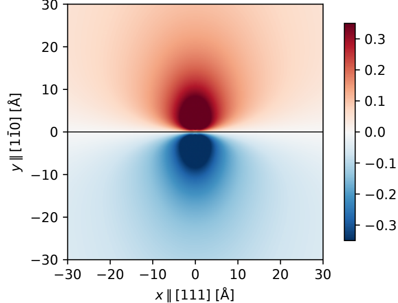
(b) U(x, y) , anisotropic Ta [eV]
