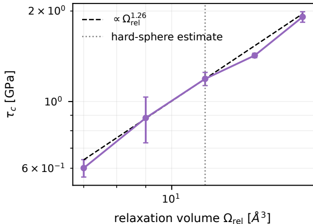
(b) relaxation volume
