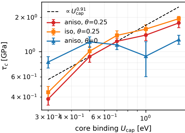
(a) core binding energy
