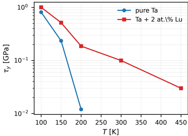
(b) kink-pair KMC: hardening at every T
