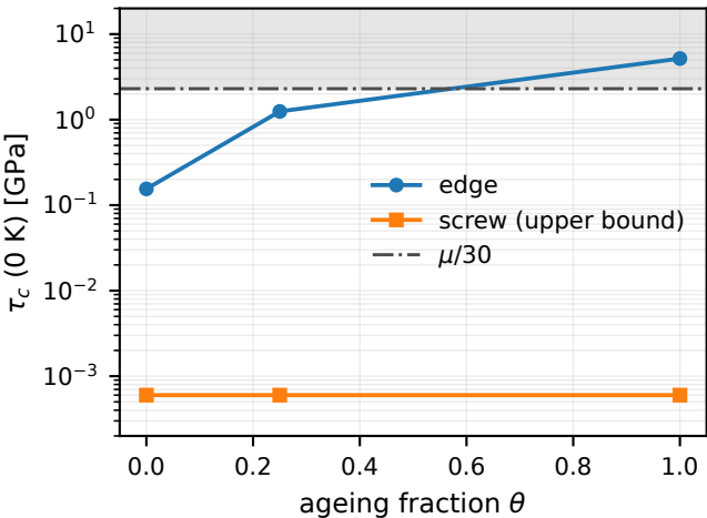
(a) the atmosphere does not pin the screw
