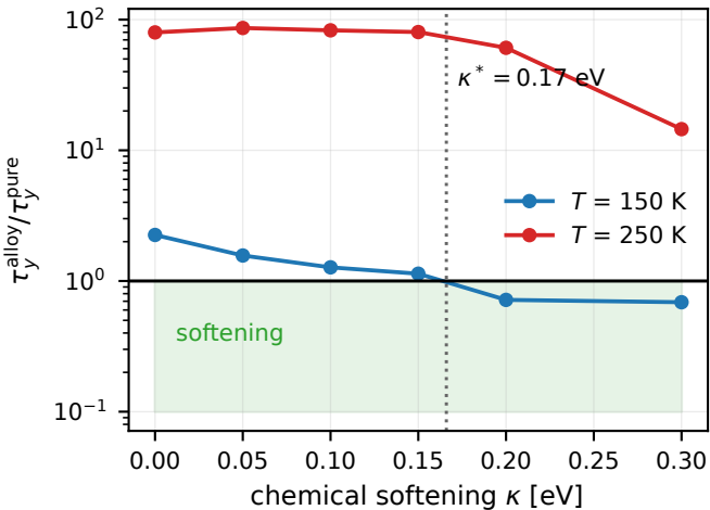
(a) threshold for softening
