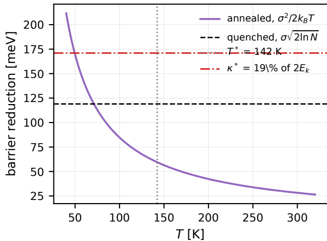
(b) what disorder can and cannot supply
