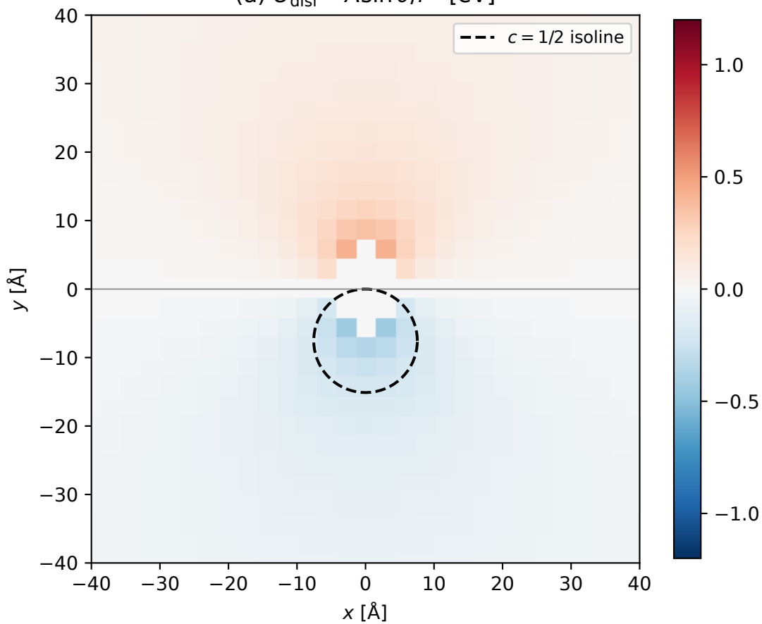
(a) U_{\text{disl}} = A \sin \theta / r [eV]
