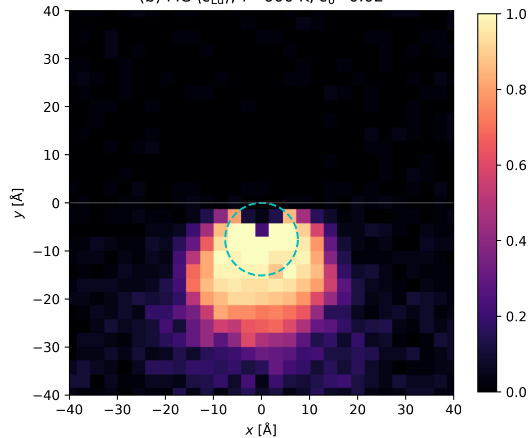
(b) MC \langle c_{\text{Lu}} \rangle , T=600 K, c_0=0.02
