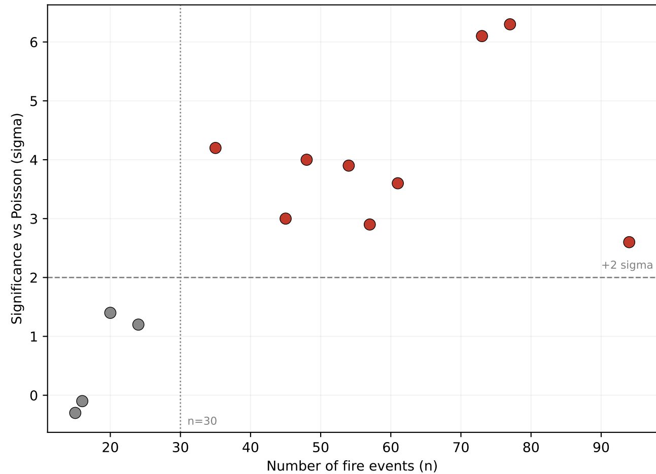
(b) Selection power of the criterion: n \geq 30 \rightarrow all significant; n < 30 \rightarrow undetermined
