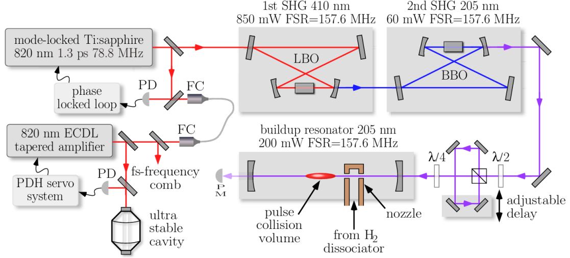
Figure 1.4: Schematic of the 1S-3S Hydrogen Spectroscopy Experimental Setup, showing the Laser System, and the spectroscopic region. PD: Photo-Detector, PDH: Pound-Drever-Hall locking scheme, FC: Fibre Coupler, ECDL: Extended Cavity Diode Laser, LBO: Lithium Triborate crystal, BBO: \beta -Barium Borate crystal, SHG: Second Harmonic Generation. Figure from [2]
