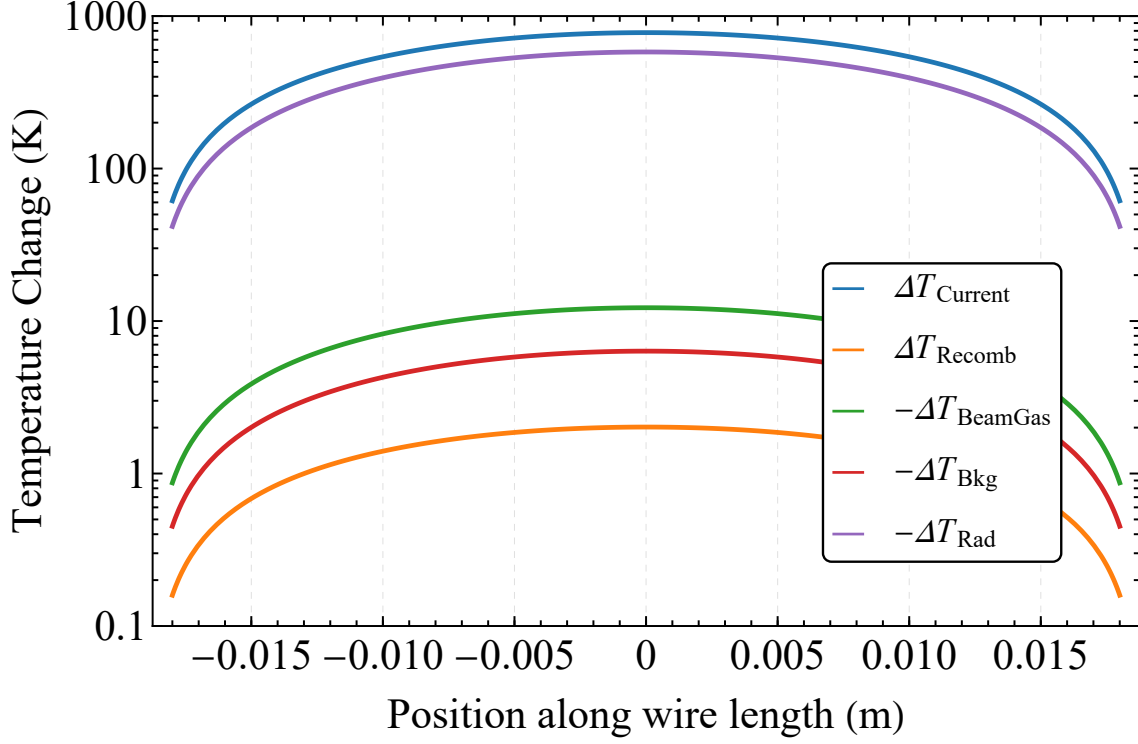
Figure 3.12: Calculation of temperature change from different heat loads by solving for steady state with conduction and probe current heating, after removing the probe current contribution, for the wire of 5 \mu m diameter. The calculations assume P_{bkg} = 1.5 \times 10^{-5} mbar, T_{bkg} = 298.15 K, T_{nozzle} = T_{beam} = 298.15 K, degree of dissociation \alpha = 0.05 and H_2 flow of 0.37 mln/min. The previously dominant cooling rate of the background gas is significantly reduced. The \Delta T_{Current} is the simulated average temperature change from the probe current which was removed from all other temperature change simulations for other heat loads, plotted to shows its large magnitude.
