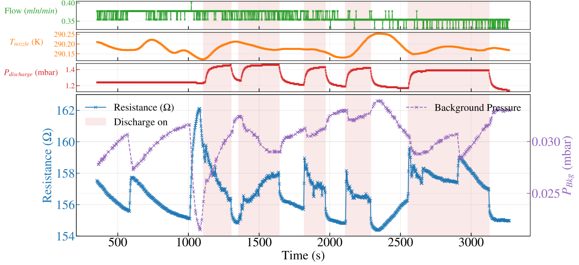
Figure 3.8: Figure shows a time sweep of different parameters in which a discharge on-off measurement for atomic hydrogen signal extraction was performed. The resistance consistently increases at plasma ignition, suggesting the presence of atomic hydrogen, but a corresponding drop in background pressure casts uncertainty on the origin of the increase in resistance.
