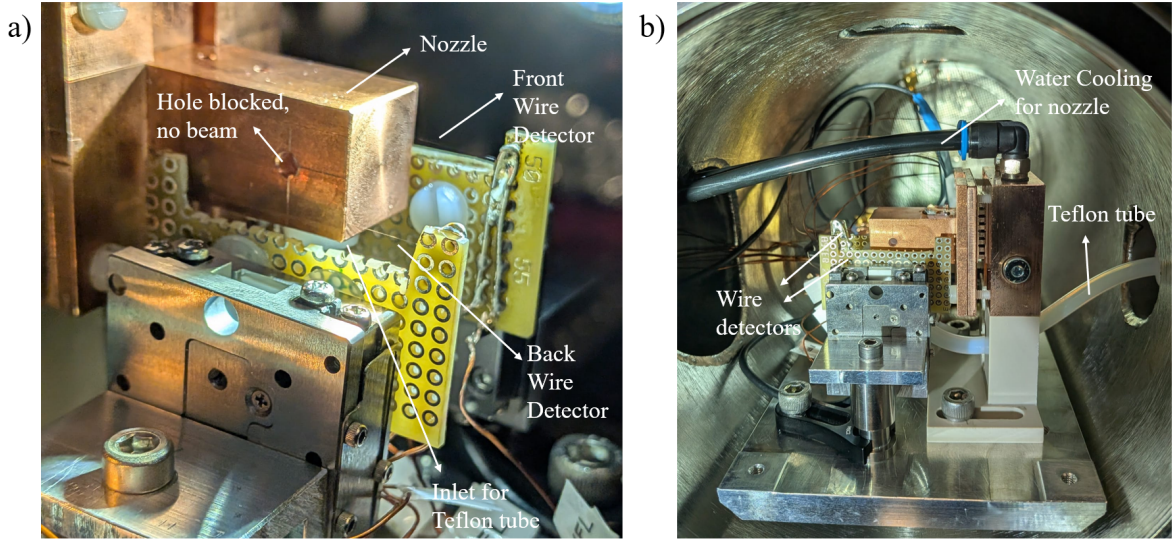
Figure 3.11: a) The front and back wire detectors with respect to the nozzle, with the nozzle back outlet blocked to block the beam. b) The nozzle and wire detector placement in the new lower-pressure chamber configuration.
