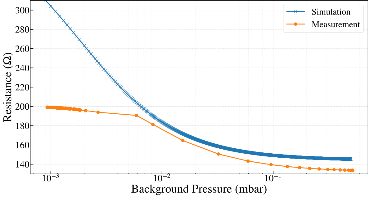
Figure 3.4: The figure shows the pressure dependence of resistance in orange, measured reproducibly while pumping or venting the chamber. The dominant background gas cooling can be explained by the steep dependence of the curve at our operating chamber pressure when the discharge is on, P_{bkg} = 1.5 \times 10^{-2} mbar. The kink observed was reproducibly present in the curve, potentially arising from another competing heat load, primarily the radiation cooling from the nozzle. The blue curve is the simulated pressure dependence of steady-state resistance after solving with conduction and probe-current heat loads. The functional dependence of the curve up to the kink matched the measurements very well, but the exact pressure and resistance values did not, potentially due to neglected heat loads and their crosstalk in the simple simulation. Simulation to reproduce the kink by adding cooling of the wire via radiation did not work out due to unknown emissivities. Both simulation and measurement are for Wire-2. The very close values of the resistance for a particular pressure above 10^{-2} mbar from measurement and simulation could be a confirmation of the consequence of the high cooling load from the high background pressure, and hence, the observed much lower resistance.
