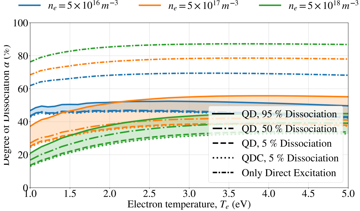
Figure 2.22: Plot depicting the uncertainties introduced to the degree of dissociation due to theory uncertainty in the value of the effective rate coefficients ratio. The top 3 lines show the degree of dissociation by including only the direct excitation channel for molecular hydrogen, at different electron densities and temperatures. Additionally, when Quenching (Q) and Dissociative Attachment (D) Channels are added, the degree of dissociation progressively falls down with increasing electron density and additionally depends on the absolute value of molecular hydrogen population ( n_{H_2} ), and hence for representative purposes, the spread due to n_{H_2} is plotted in terms of 3 values of degree of dissociation (95 %, 50 % and 5 %) corresponding to 3 values of n_{H_2} ( 2 \times 10^{20} , 3 \times 10^{21} and 8 \times 10^{21} \text{ m}^{-3} ). All of these values correspond to a single plasma emission spectrum, labelled "A" in Fig. 2.18, and all include only the Fulcher Intensity from the "Integrating" method with a T_{vib}(X^1) = 5000 \text{ K} used for extrapolation.
