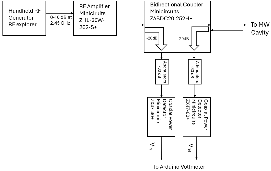
Figure D.1: Electrical Schematic for MW application to discharge Cavity
