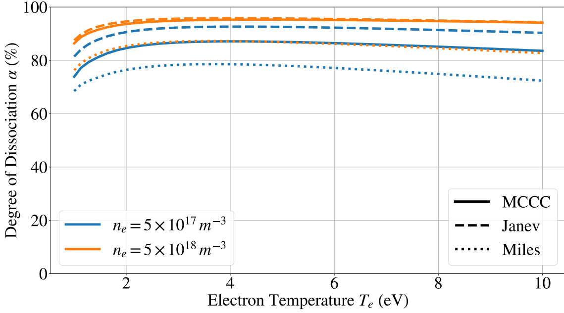
Figure 2.21: Variance in the degree of dissociation of a single plasma spectrum (labelled spectrum A in Fig. 2.18), with change in electron temperature and density, with the 3 collisional cross-sectional databases available in H_2 Yacora model: Miles[35], Janev [36] and MCCC [23]. Only two values of n_e are shown for representative purposes. Dummy values of T_{H_2} = 500 \text{ K} and T_{vib}(X^1) = 5000 \text{ K} used.
