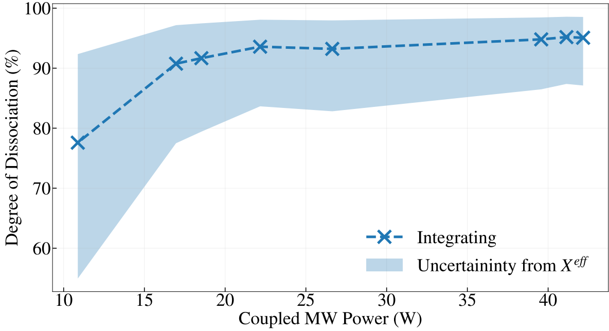
Figure 2.19: Change in degree of dissociation when the MW power applied to the cavity was varied. For each applied power, the data with the most power coupled was chosen. Fulcher intensities are obtained only by "Integrating", and the rate coefficients for Fulcher emission are taken from the MCCC cross-sectional database in the direct excitation channel of the molecular H_2 model in Yacora. Additionally, due to unknown values of plasma parameters, the rate coefficients used for calculations were a middle value in the range and an errorbar was added according to the extreme values of rate coefficients for the relevant range of plasma parameters. These values are the same as those mentioned in Fig. 2.18.
