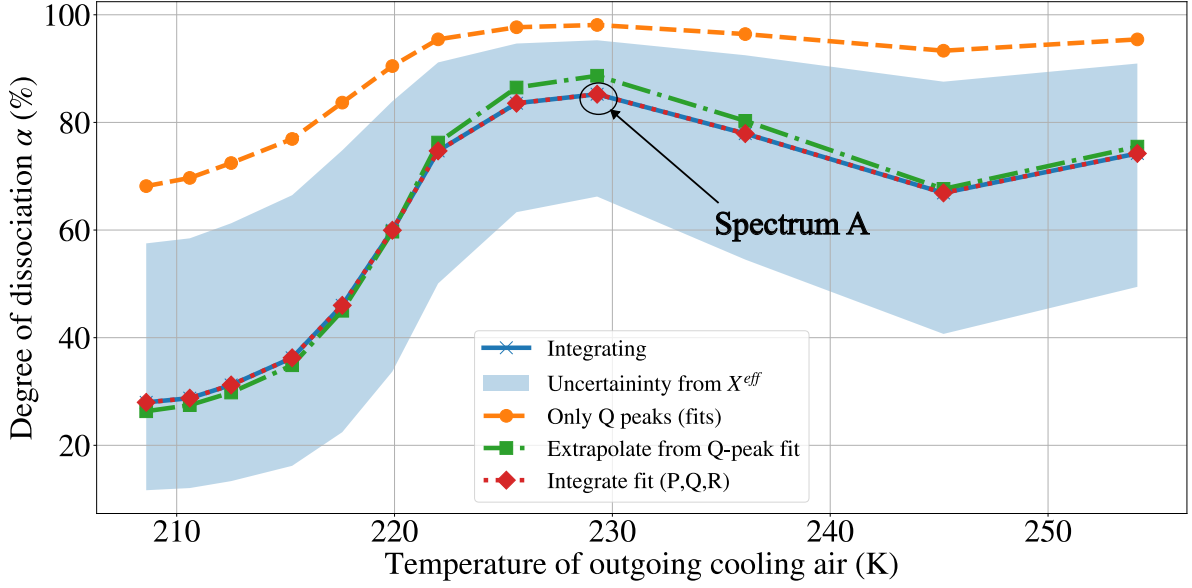
Figure 2.18: Plot shows the change in dissociation fraction in our hydrogen plasma when the discharge temperature is varied. All data taken at H_2 flow of \approx 0.37 \text{ mln/min} with 30 W of MW power applied. The degree of dissociation was calculated from Fulcher intensities from all four intensity methods (Sec. 2.5). It is clear here that estimating the degree of dissociation using only the Q-line emission overestimates it by a large margin. Additionally, due to unknown values of plasma parameters, the rate coefficients used for calculations were as follows: the curves for each method use T_e = 7.85 \text{ eV} , n_e = 5 \times 10^{17} \text{ m}^{-3} and T_{vib}(X^1) = 5000 \text{ K} , which corresponds to X_{ratio} = 0.1705 , whereas the shaded region represents the spread of the curves when the plasma parameters vary. In particular, the upper boundary corresponds to T_e = 3.79 \text{ eV} , n_e = 5 \times 10^{18} \text{ m}^{-3} and T_{vib}(X^1) = 1000 \text{ K} , which corresponds to X_{ratio} = 0.0489 , while the lower boundary corresponds to T_e = 1 \text{ eV} , n_e = 5 \times 10^{16} \text{ m}^{-3} and T_{vib}(X^1) = 12000 \text{ K} , which corresponds to X_{ratio} = 0.5023 . The MCCC cross-sectional database with only direct excitation channels was used for the calculation in Yacora. Spectrum A is the spectrum used for the calculation of uncertainties in the degree of dissociation, in Sec. 2.6.3
