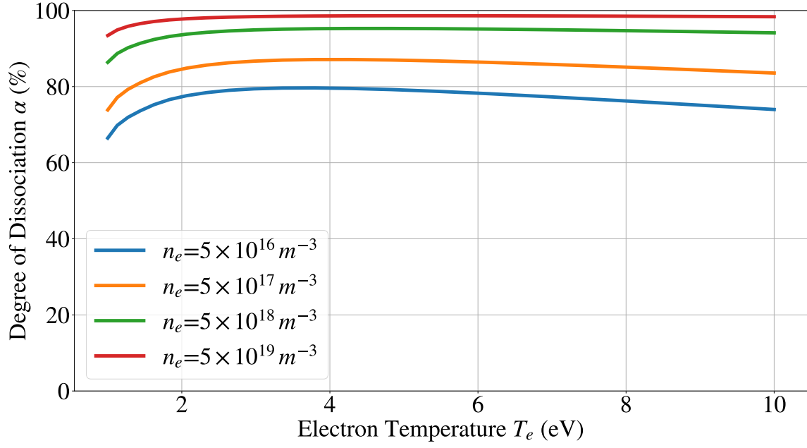
Figure 2.20: Variance in Degree of Dissociation of a single plasma spectrum (labelled spectrum A in Fig. 2.18), with change in electron temperature and density, when the cross-sectional database for the H_2 model in Yacora was chosen to be MCCC [23]. Dummy values of T_{H_2} = 500 \text{ K} and T_{vib}(X^1) = 5000 \text{ K} are used.
