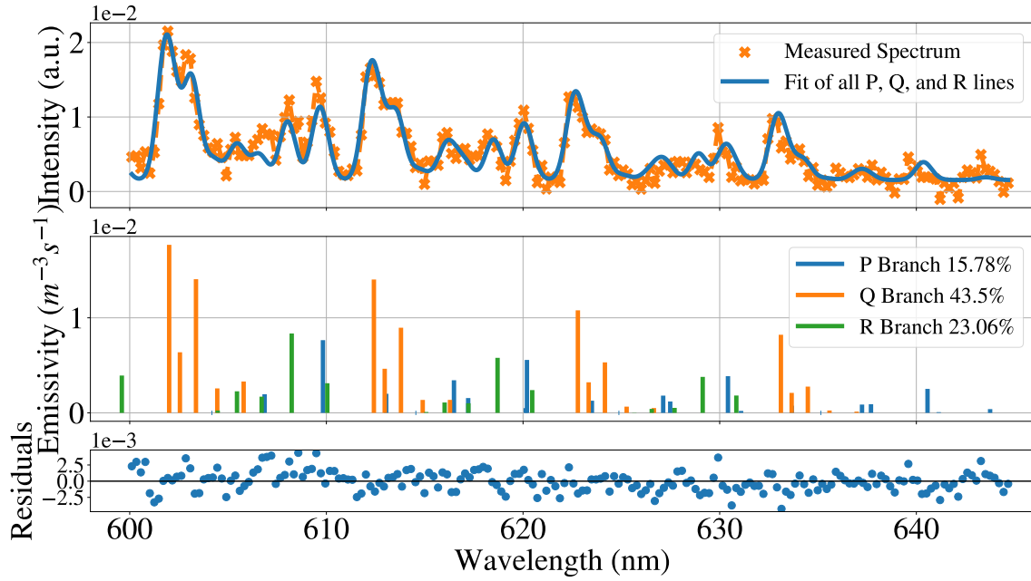
Figure 2.15: Fit of all P, Q, and R emissions for the first four vibrational bands of the measured Fulcher spectrum, and the corresponding calculated lines used for fitting. The method, after extrapolation, is termed as "Integrate fit (P, Q, R)".
