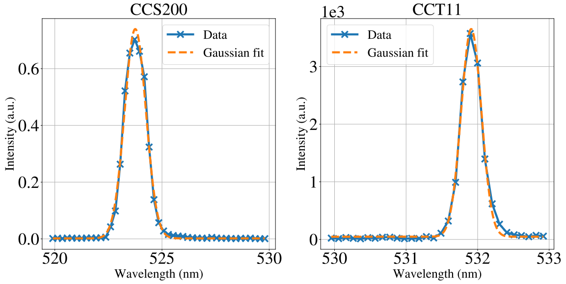
Figure C.3: Spectrum of output of Coherent Verdi V-18 at 532 nm with a) Thorlabs CCS200 Spectrometer 1 , and b) Thorlabs CCT11 Spectrometer and a Gaussian fit to both, in an attempt to find the point spread function of the spectrometers.
