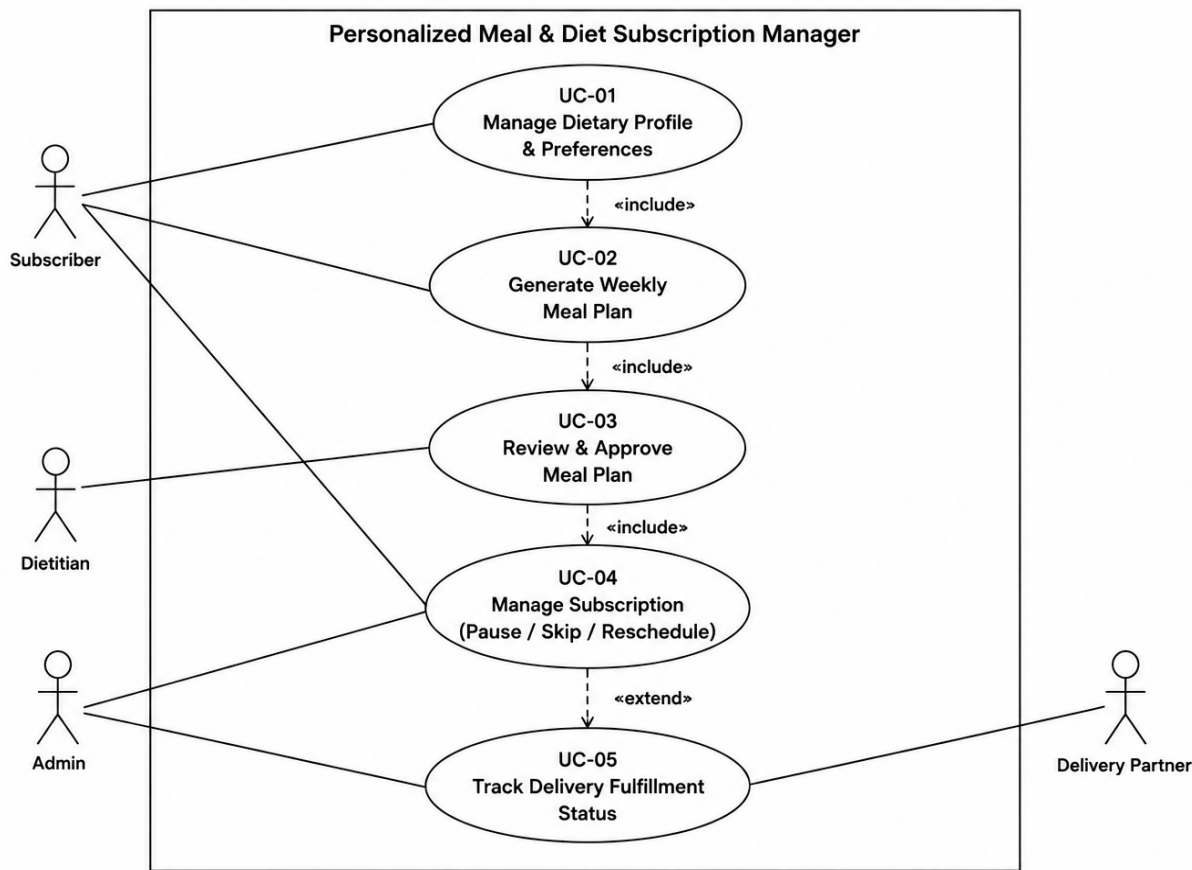
UML Use-Case Diagram - Personalized Meal & Diet Subscription Manager
