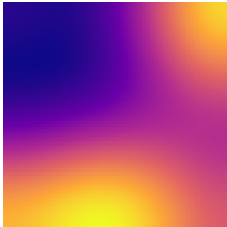
True field
