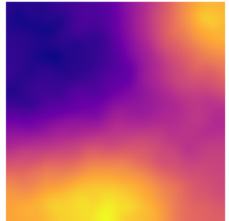
Fourier prediction
