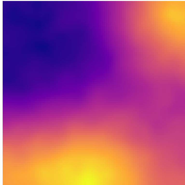
SAR prediction
