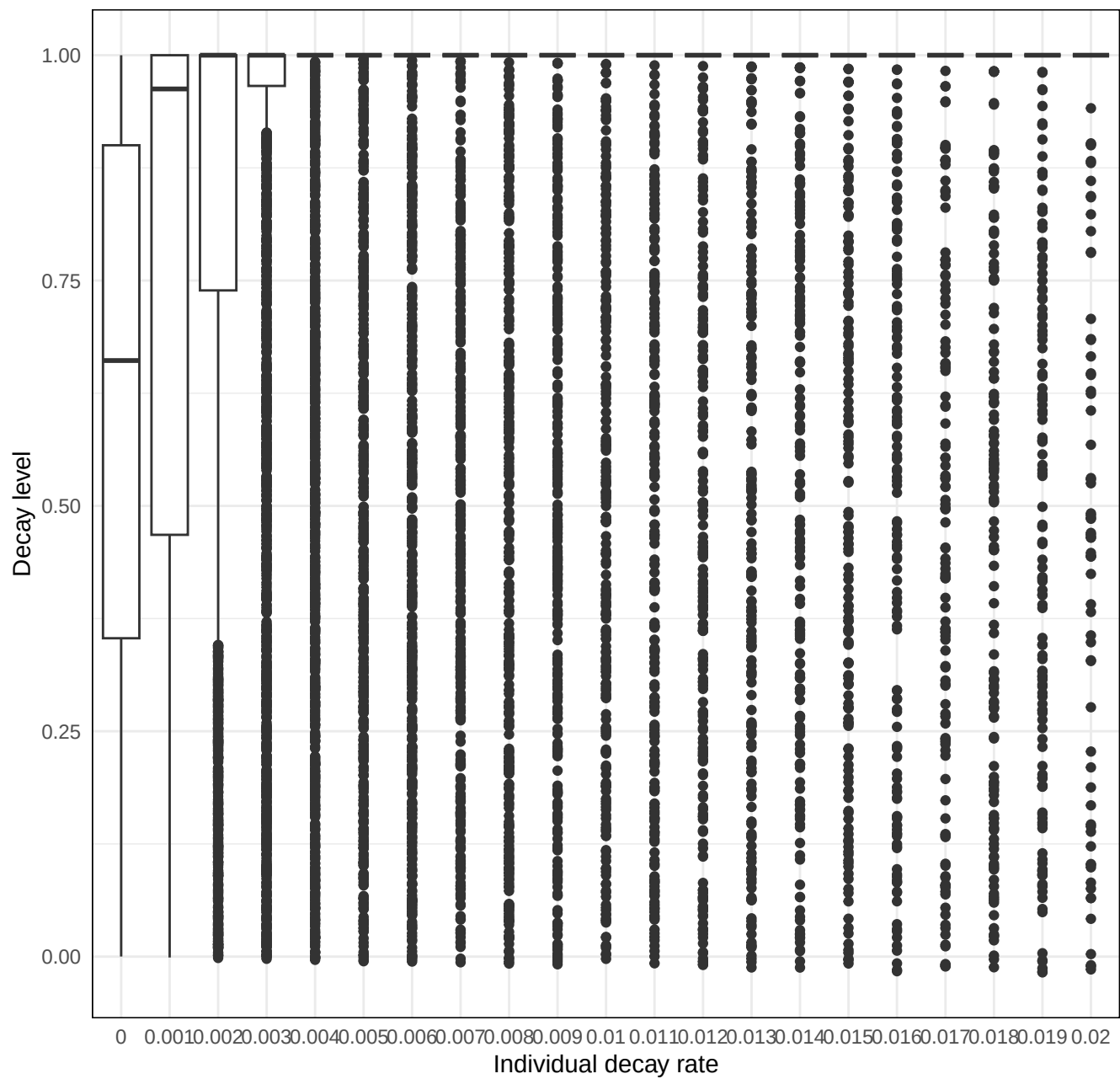
Taphonomy Simulator – Randomised decay rate vs preservation
