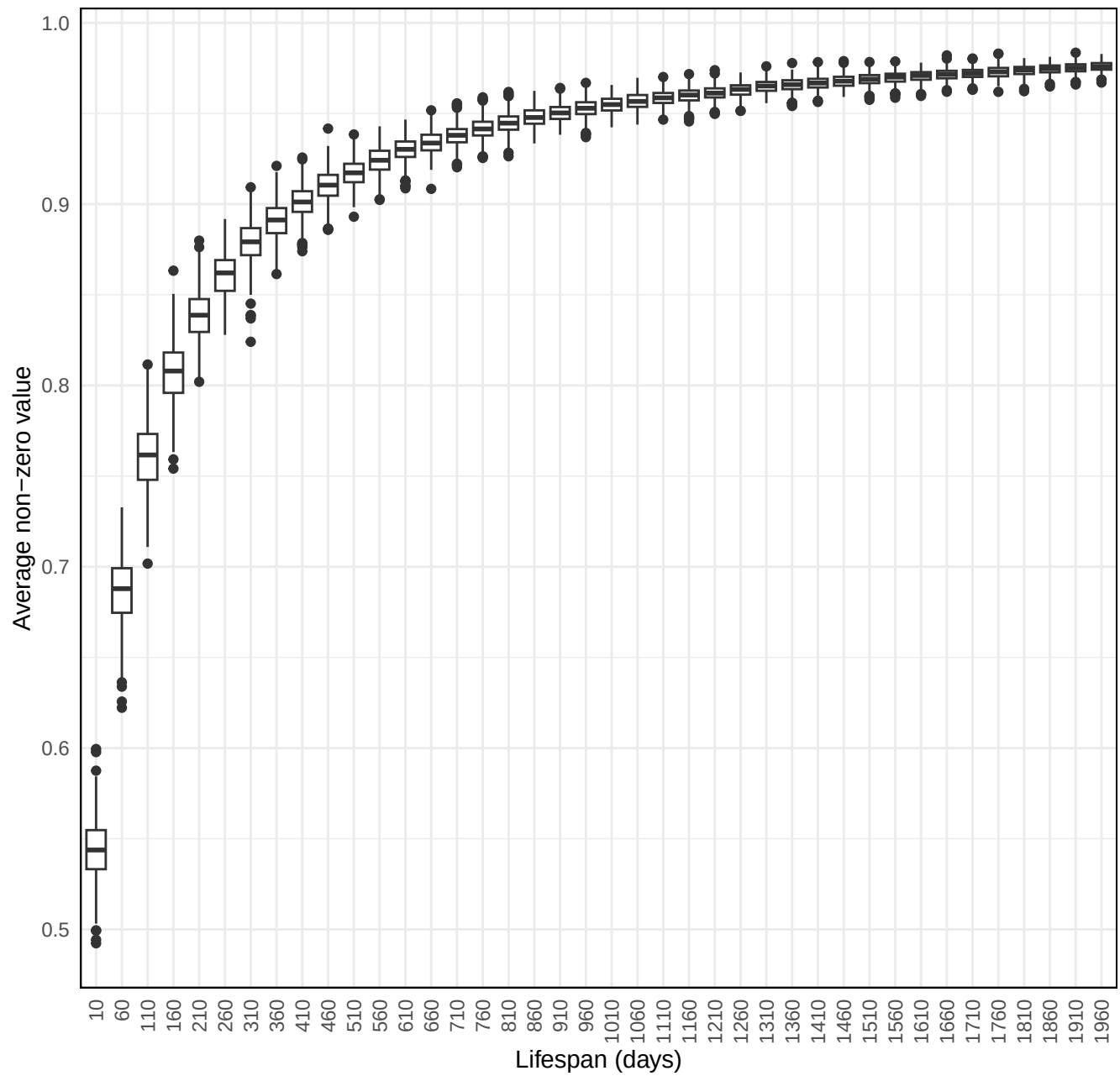
Taphonomy Simulator – lifespan vs preservation
