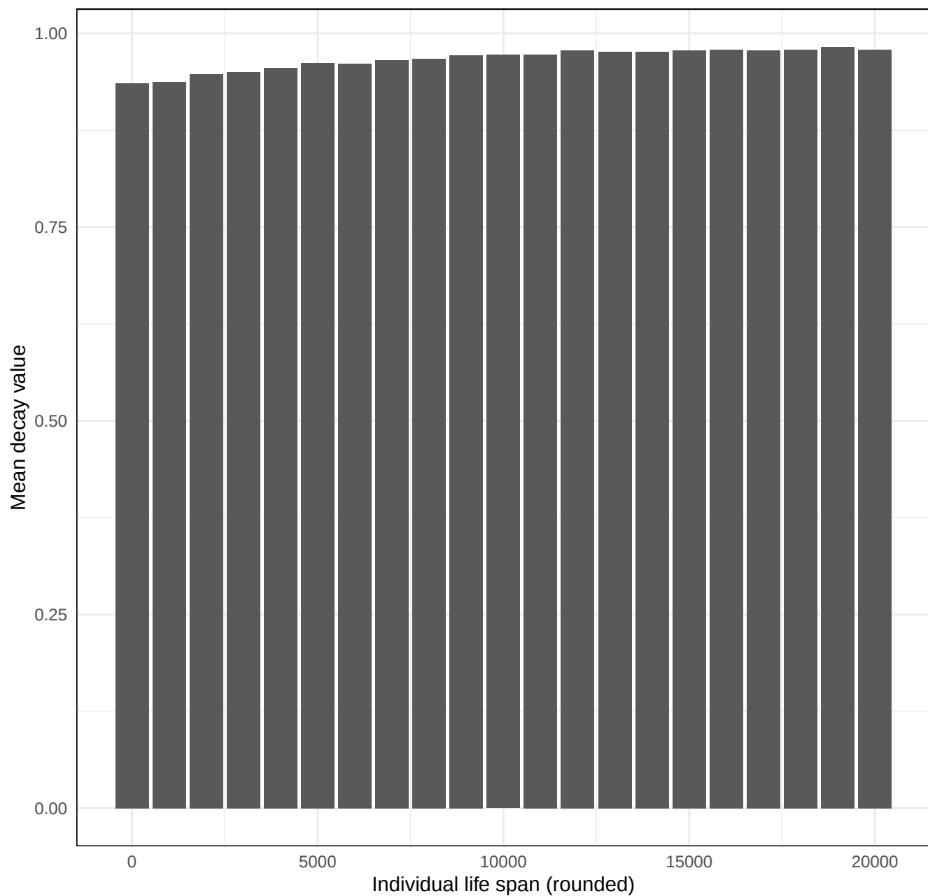
Taphonomy Simulator – Randomised lifespan vs mean decay
