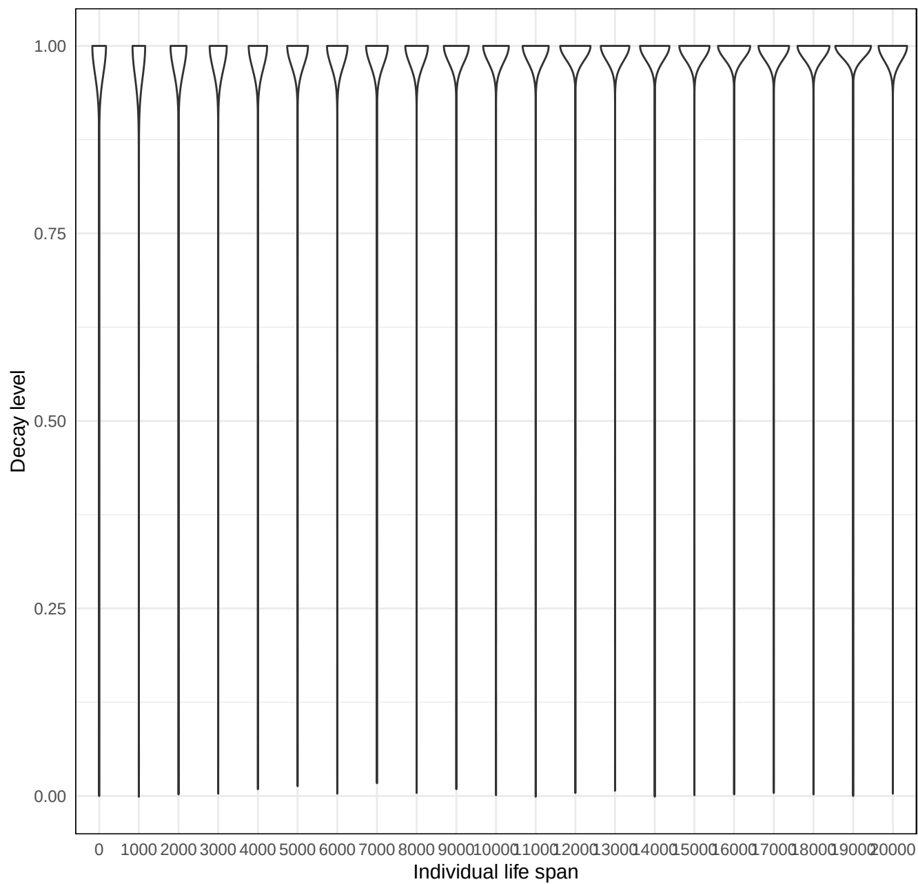
Taphonomy Simulator – Randomised life span vs preservation
