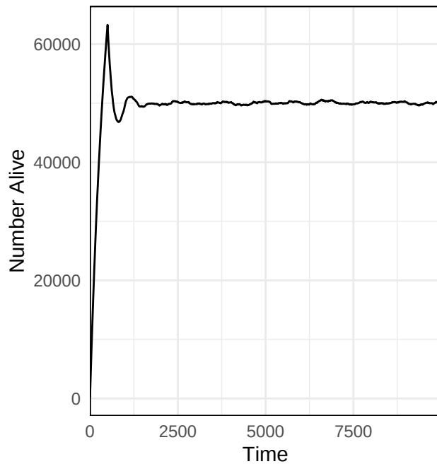
Taphonomy Simulator – Number Alive
