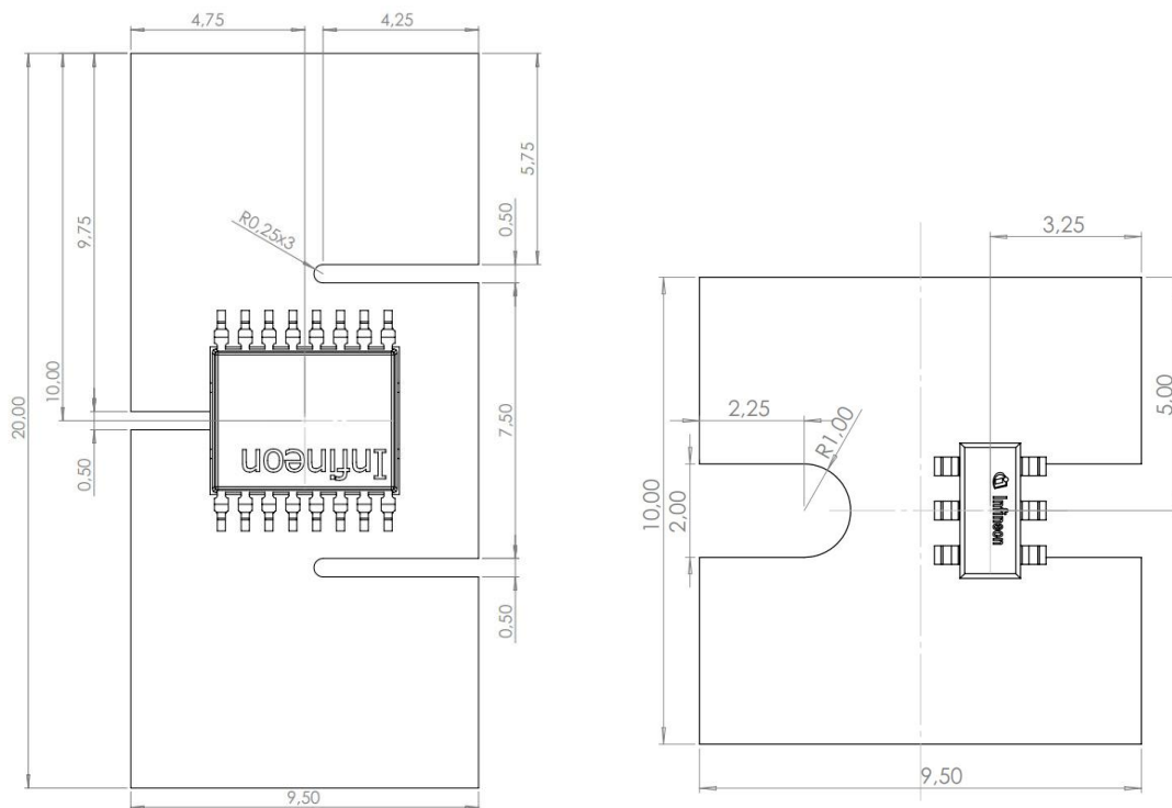
Sensor position on a power rail. Dimensions in millimetres
