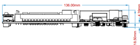
View from Front side (Scale 1:1)
