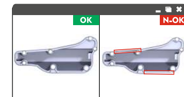
SEALANT INSPECTION
