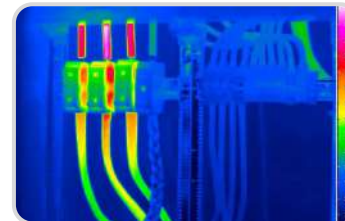
THERMAL INSPECTION OF CABLE
