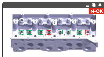
VALVE SEAT INSPECTION
