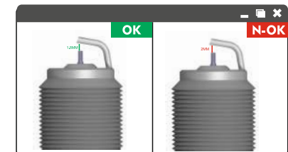
SPARK PLUG GAP INSPECTION
