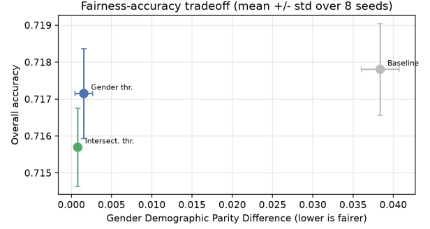
Fig. 4. Gender fairness–accuracy tradeoff (mean \pm std over eight seeds). Threshold calibration reaches near-zero DPD at a small accuracy cost.
