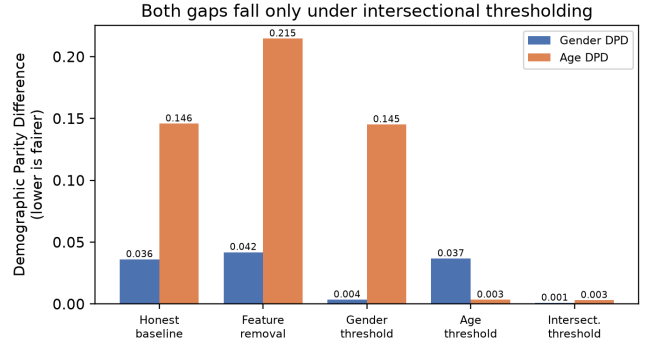
Fig. 2. Demographic parity difference for both protected attributes across the five configurations (seed 42). Feature removal worsens the age gap; single-attribute thresholds mitigate only their own attribute; intersectional thresholding reduces both.
