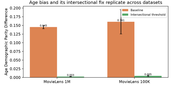
Fig. 5. The substantial baseline age gap and its intersectional mitigation replicate on the independent MovieLens 100K dataset (mean \pm std over eight seeds).
