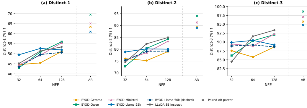
Figure 5: Sliding model-token Distinct-1/2/3 for the final models across diffusion inference budgets. Crosses show the paired AR parents; BYOD-Llama-25k and BYOD-Llama-50k share the same parent. Higher-order metrics show the same broad diversity pattern while compressing differences because longer n -grams are less likely to repeat exactly.
