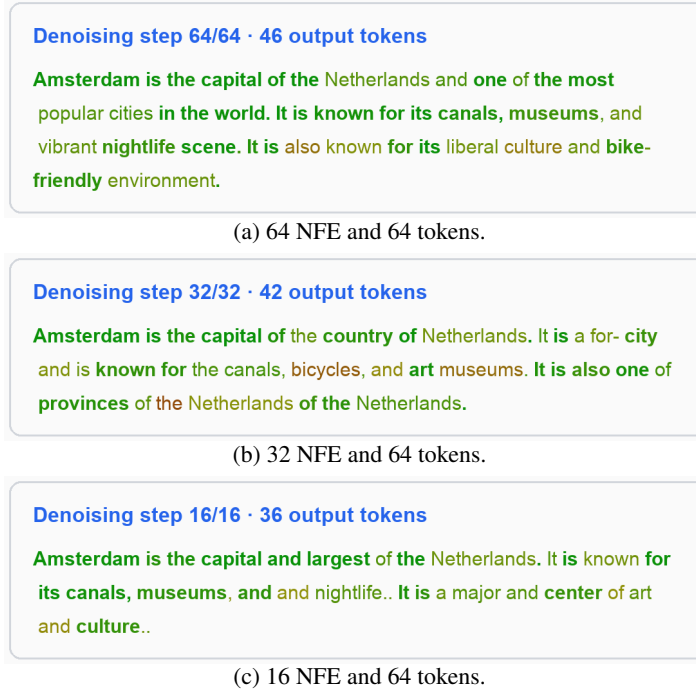
Figure 7: Confidence-guided BYOD-Gemma-2-9B trajectories at decreasing inference budgets on a 64-token canvas. Red-to-green coloring records each retained token’s sampling probability.
