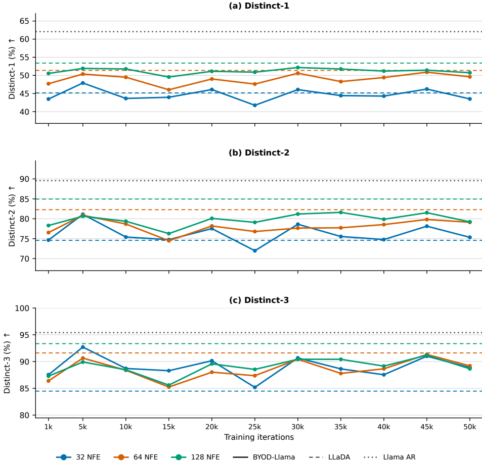
Figure 6: Sliding model-token Distinct-1/2/3 throughout BYOD-Llama-50k training. Solid colored lines are BYOD-Llama checkpoints at each NFE budget; matching dashed lines are fixed LLaDA references, and the dotted gray line is Llama AR. All three metrics fluctuate across checkpoints without a strong monotonic trend.
