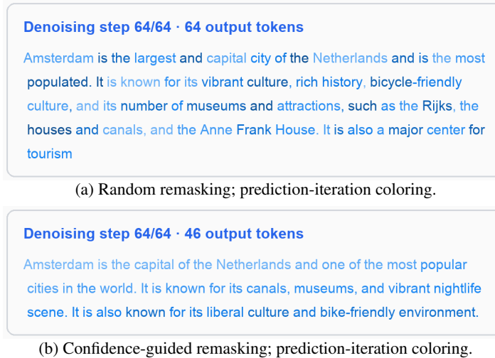
Figure 8: Remasking comparison for BYOD-Gemma-2-9B at 64 NFE on a 64-token canvas. Blue intensity records the iteration at which each retained token was predicted.
