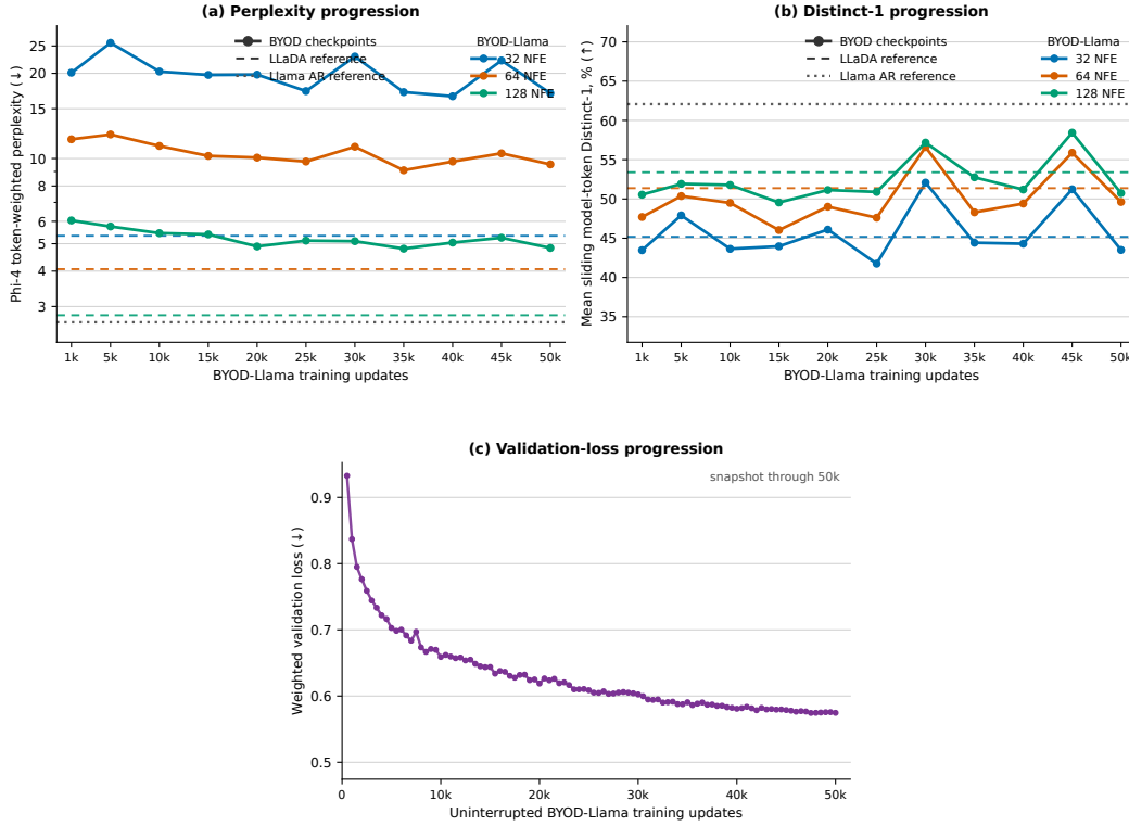
Figure 2: BYOD-Llama training diagnostics. (a) Token-weighted Phi-4 perplexity for 128-token generations, shown on a logarithmic y-axis. (b) Mean sliding model-token Distinct-1 for the same generations, reported as a percentage. Each NFE series contains 100 prompts at all eleven checkpoints from the uninterrupted llama-3.1-8b-mask-long run. Color-matched dashed lines are fixed LLaDA references; the dotted gray line is the unchanged Llama AR parent measured over the same 100 prompts. (c) Weighted validation loss from the uninterrupted run through 50k updates. Lower is better in (a,c), and higher is better in (b).
