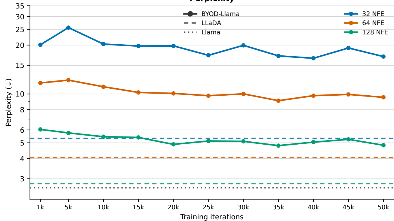
Perplexity
