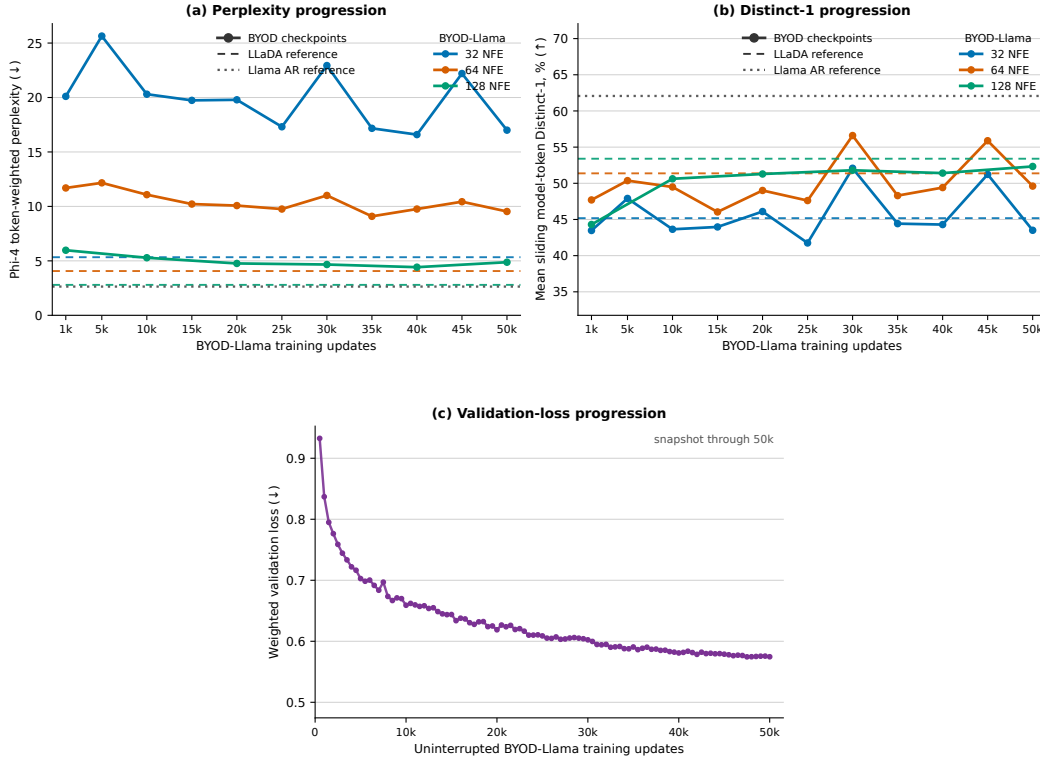
Figure 2: BYOD-Llama training diagnostics. (a) Token-weighted Phi-4 perplexity for 128-token generations. (b) Mean sliding model-token Distinct-1 for the same generations, reported as a percentage. The 32- and 64-NFE series contain all eleven checkpoints from the uninterrupted llama-3.1-8b-mask-long run; the retained 128-NFE series combines the initial run through 20k with effective 30k/40k/50k checkpoints from the continued run. Color-matched dashed lines are fixed LLaDA references; the dotted gray line is the unchanged Llama AR parent measured over 100 prompts. (c) Weighted validation loss from the uninterrupted run through 50k updates. Lower is better in (a,c), and higher is better in (b).
