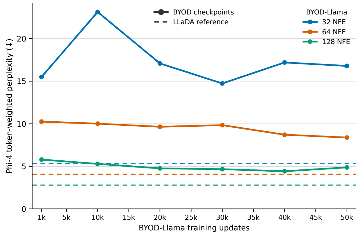
(a) Perplexity progression
