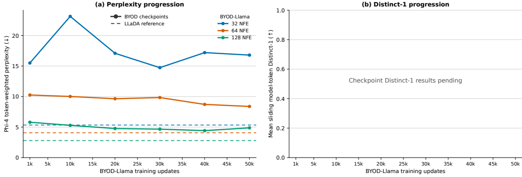
Figure 2: Provisional checkpoint-wise diagnostics for 128-token BYOD-Llama generations, with fixed LLaDA references at 32, 64, and 128 NFE. (a) Token-weighted Phi-4 perplexity (lower is better). (b) Mean sliding model-token Distinct-1 (higher is less repetitive); checkpoint values are pending and the panel is wired to the same workbook-driven plotting pipeline. Solid marked lines denote BYOD checkpoints and color-matched dashed lines denote LLaDA. Blank cells are omitted rather than interpolated.
