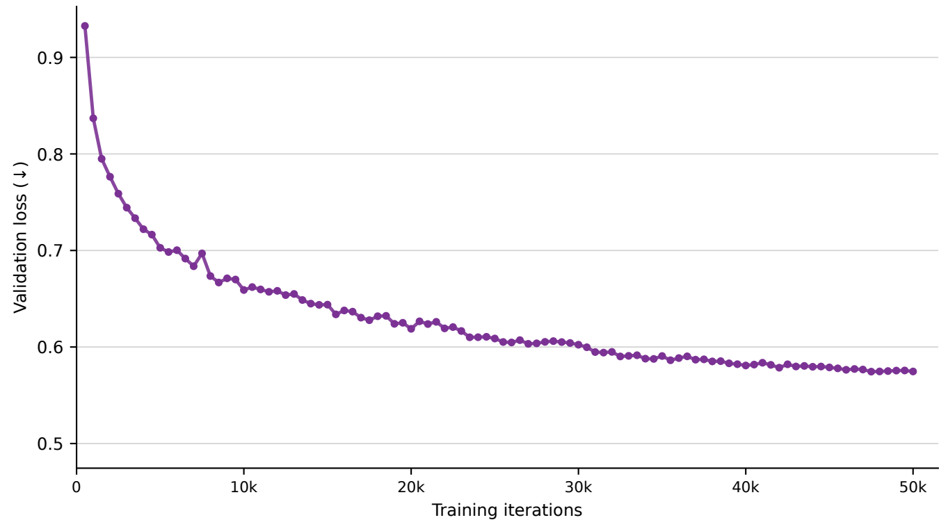
Validation loss
