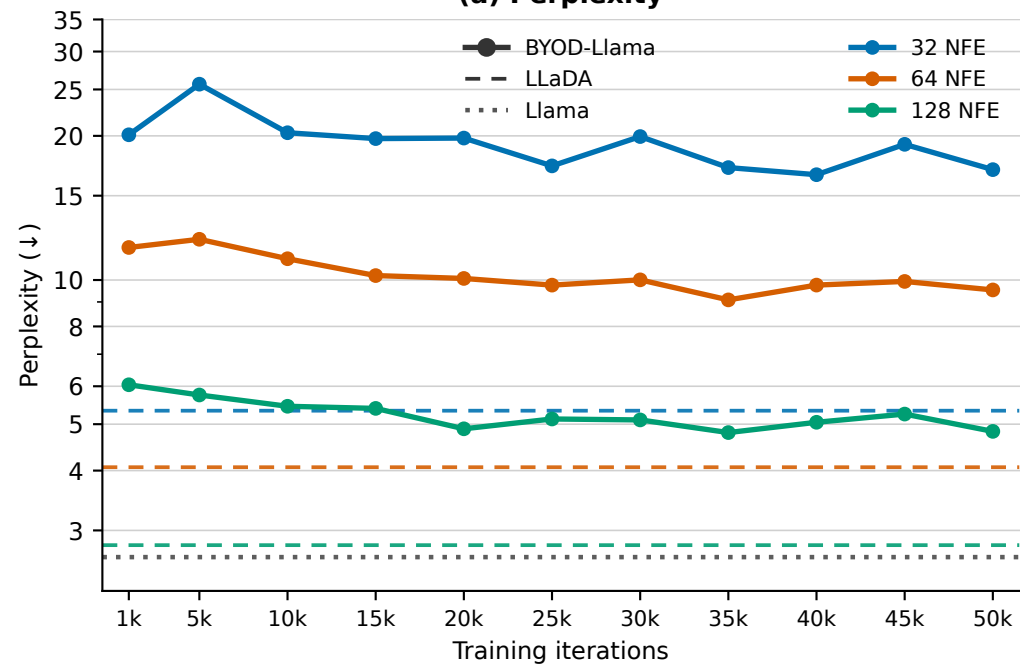
(a) Perplexity
