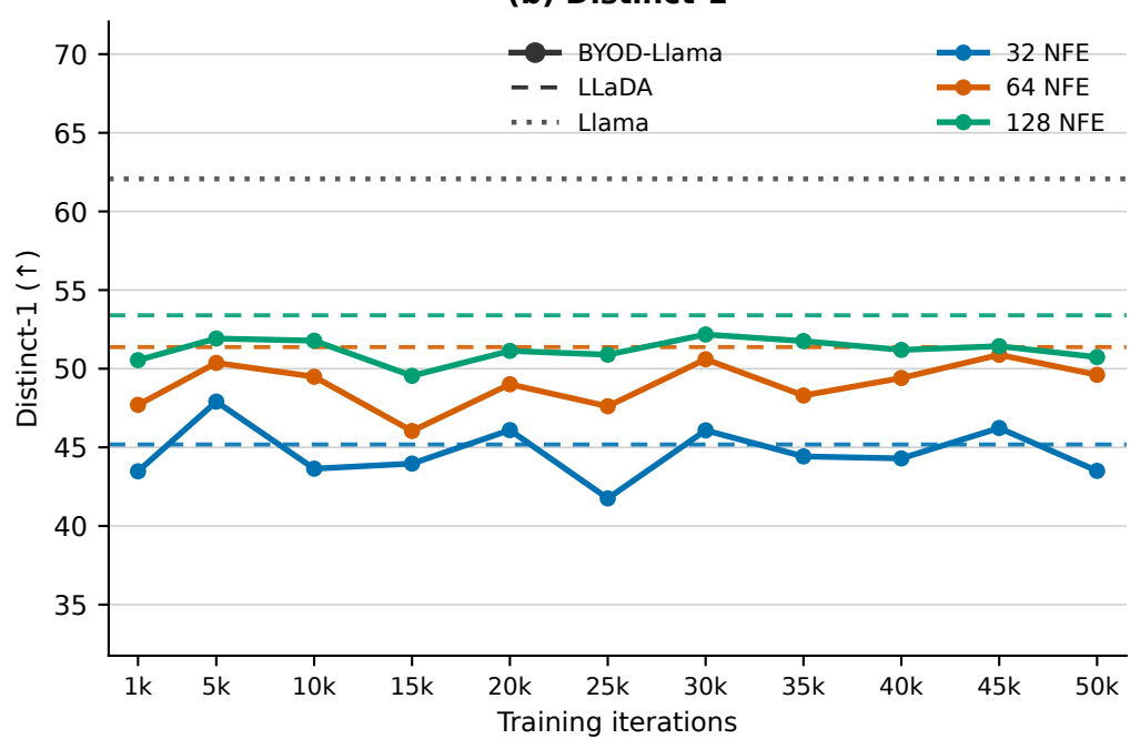
(b) Distinct-1
