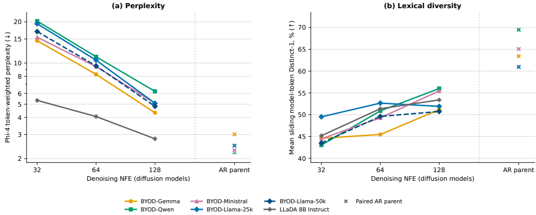
Figure 3: Visualization of the open-generation results in Table 4. Lines connect each diffusion model’s results at 32, 64, and 128 NFE; crosses to the right show the corresponding AR-parent reference without treating AR decoding as an NFE condition. BYOD-Llama-25k and BYOD-Llama-50k share one AR parent, and LLaDA has no paired AR reference. Perplexity is shown on a logarithmic axis.
