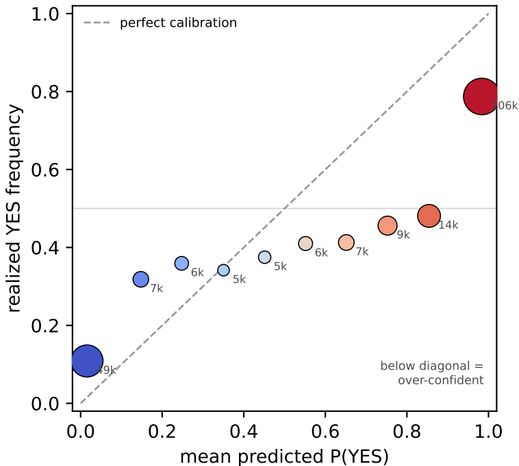
Settlement-head reliability (Brier 0.206)
