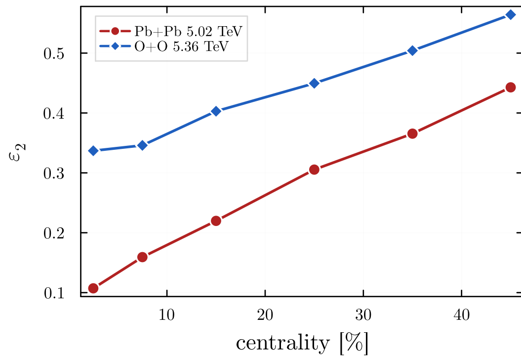
(a) initial eccentricity
