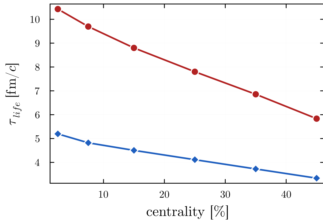
(b) fireball lifetime
