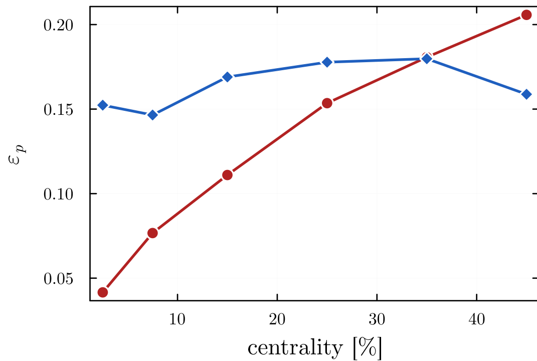
(c) momentum anisotropy, saturated
