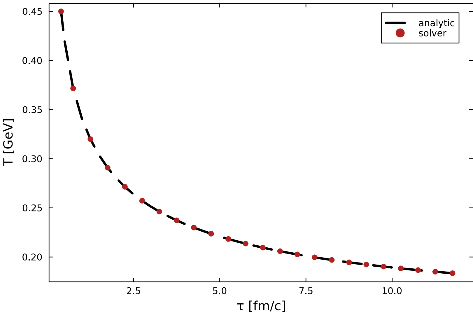
Bjorken — exact (max rel. err 9.3e-05)
