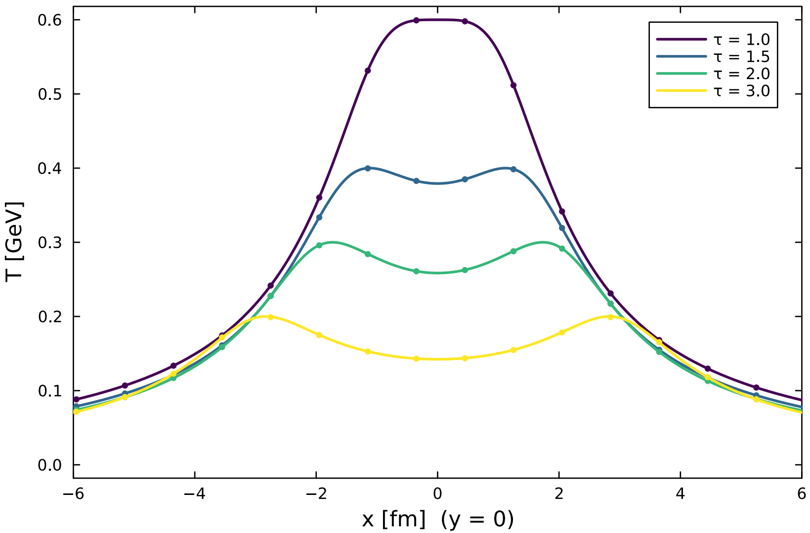
Gubser ideal — lines exact, points solver (order 1.96)
