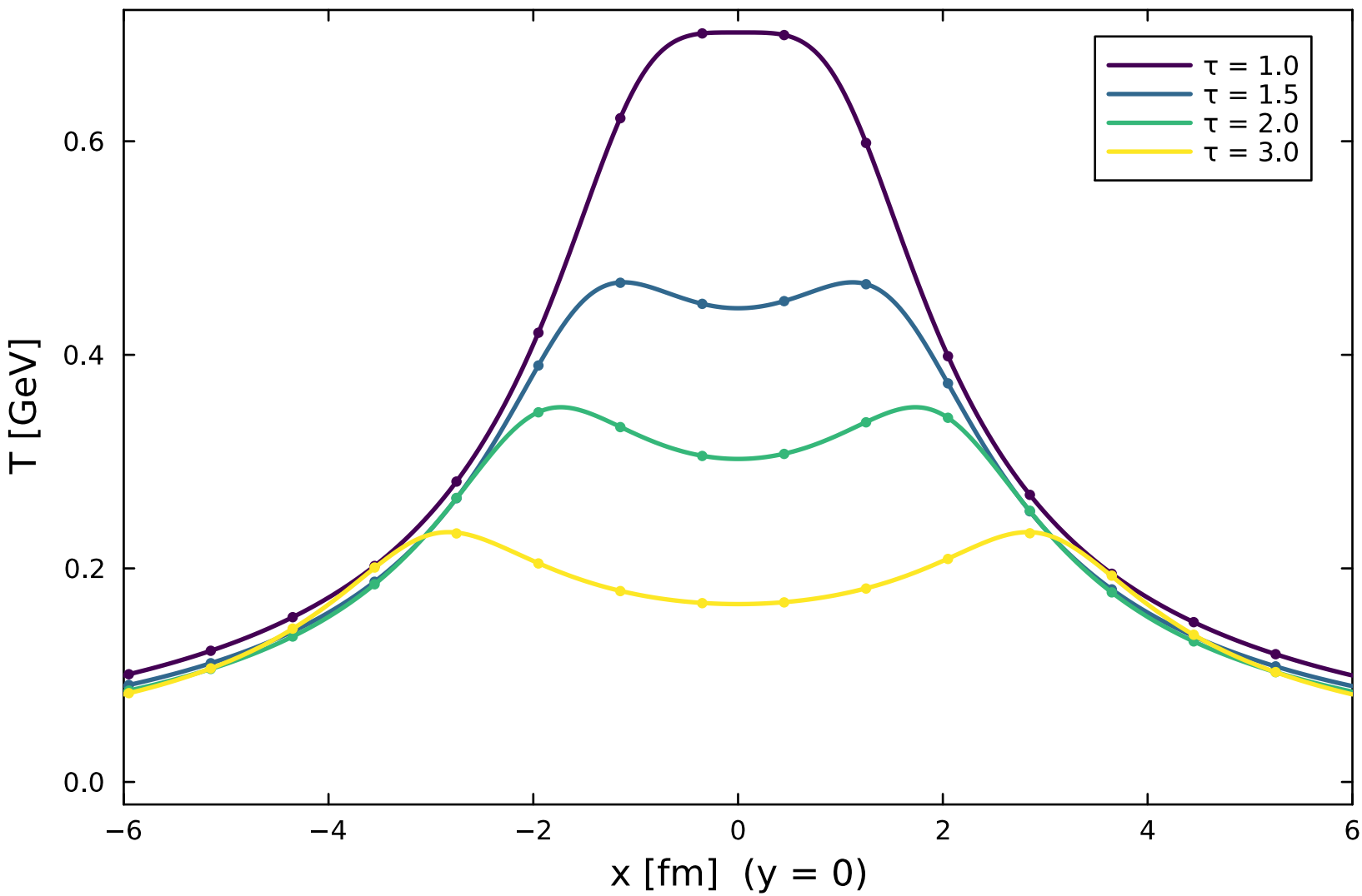
Gubser viscous \eta/s=0.02 — lines exact, points solver (order 2.00)
